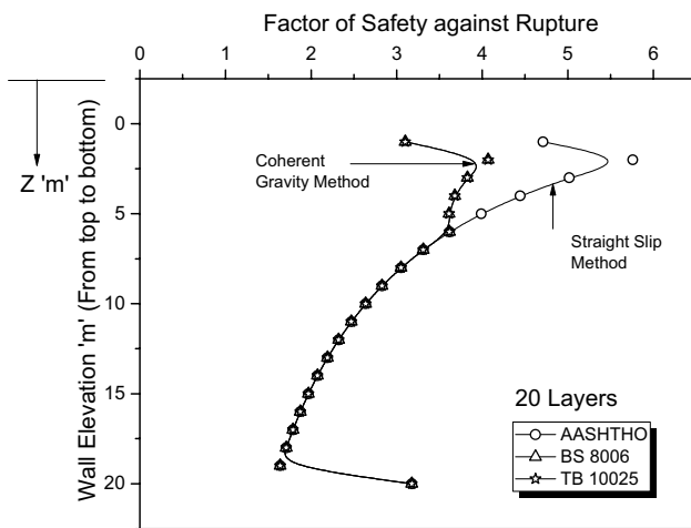
Fig. 6 FS against rupture as per AASHTO, BS 8006 and TB 10025
