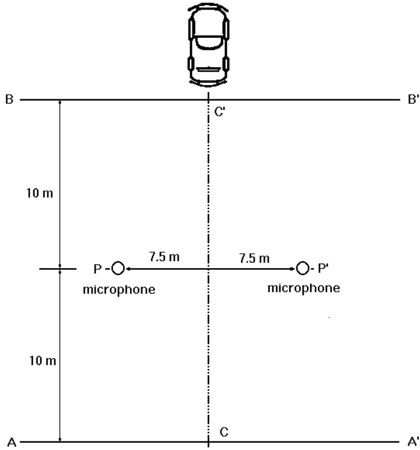
Figure 1: Microphone positions for the measurement
