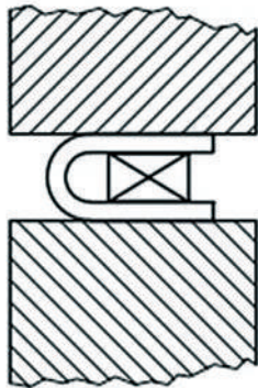
Figure — Bending the Legs of the Test Piece
