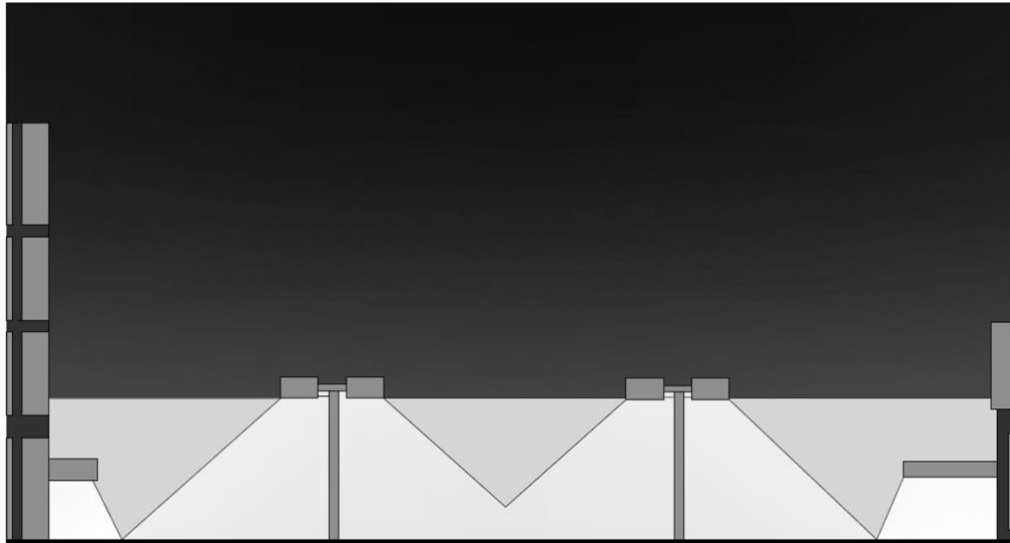
FIG. 12 FACADE LIGHTING USING SHIELDED FIXTURES
