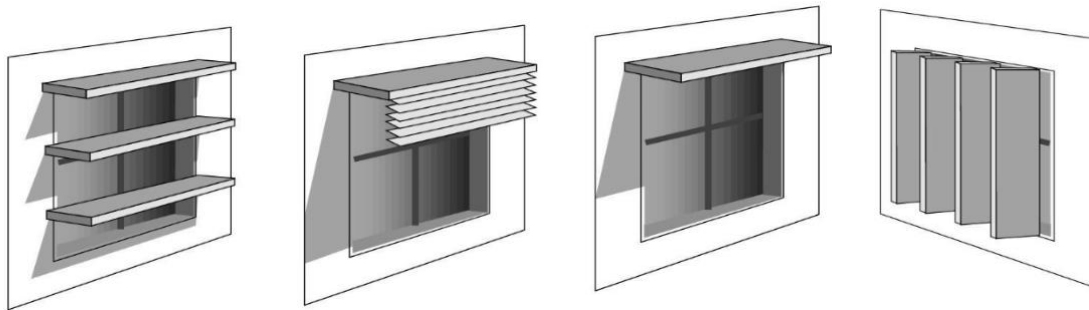
FIG. 19 COMMONLY USED SHADING DEVICES
