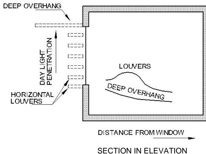
FIG. 22 COMPARISON OF DAYLIGHT PENETRATION WITH USE OF TWO SHADING DEVICES NAMELY DEEP OVERHANGS AND LOUVERS
