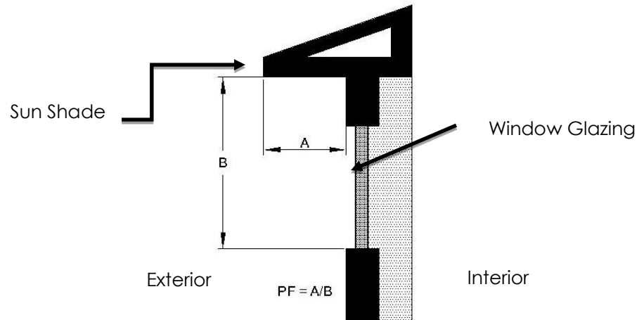
FIG. 15 PROJECTION FACTOR FOR HORIZONTAL OVERHANG FOR A TYPICAL WINDOW SECTION
