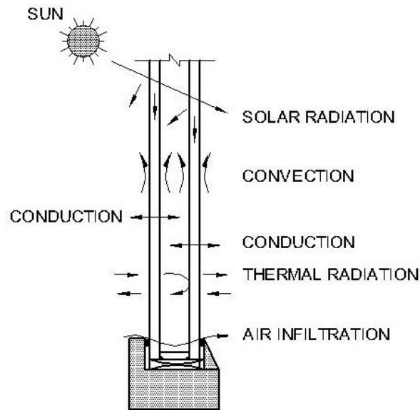
FIG. 14 TYPICAL FLOW OF SOLAR HEAT AND AIR INFILTRATION THROUGH A GLAZED WINDOW SECTION
