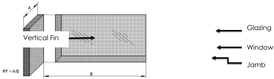
FIG. 16 PROJECTION FACTOR FOR VERTICAL FIN
