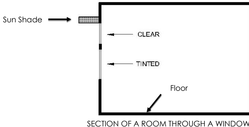
FIG. 18 ARRANGEMENT SHOWING VISION WINDOW AREA AND DAY LIGHT WINDOW AREA
