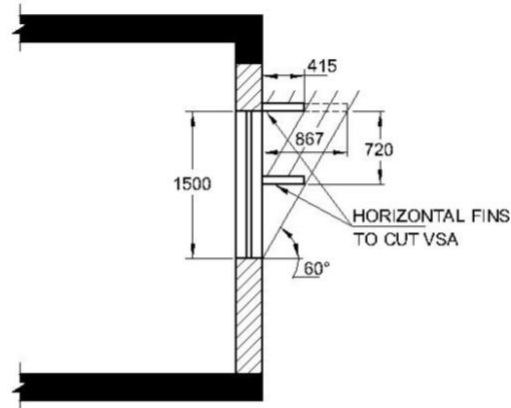
SECTION IN ELEVATION
