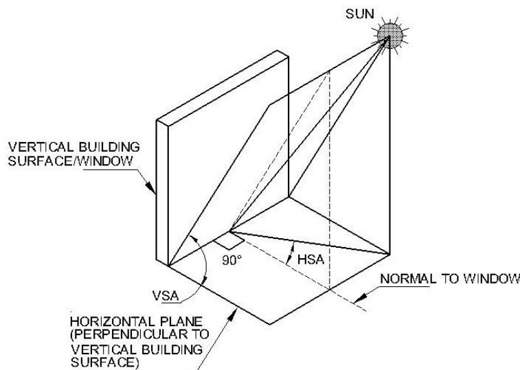
FIG. 1 HORIZONTAL AND VERTICAL SOLAR ANGLE FORMULATION
