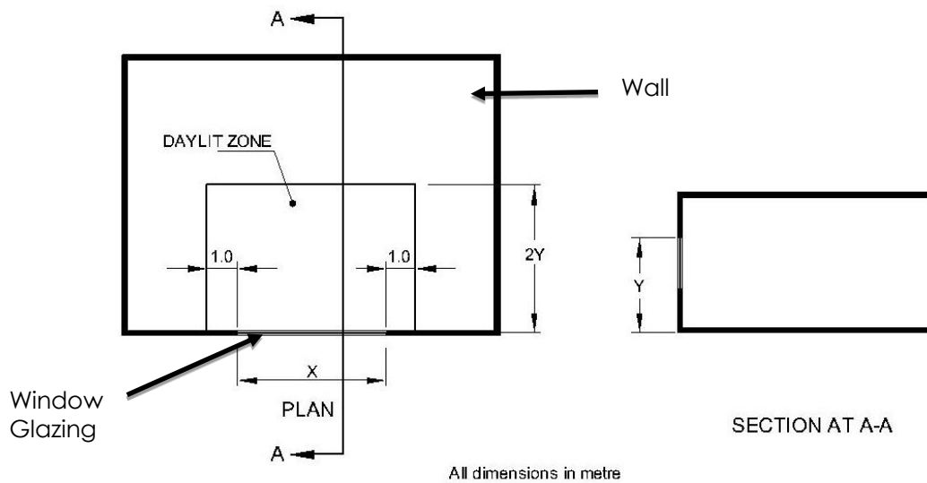
FIG. 17 DAY-LIT PERIMETER ZONE ASSOCIATED TO A WINDOW
