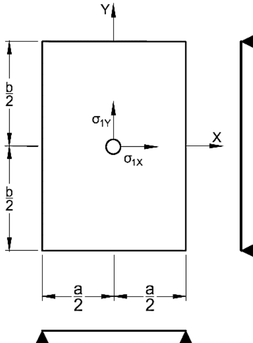
FIG. 6 ALL EDGES SIMPLY SUPPORTED
