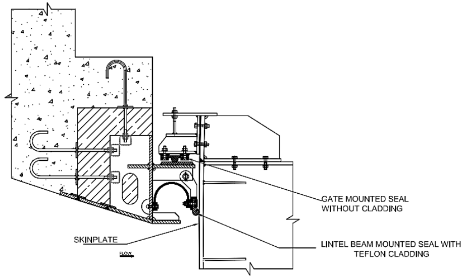
(E) TOP SEAL WITH SKIN PLATE
