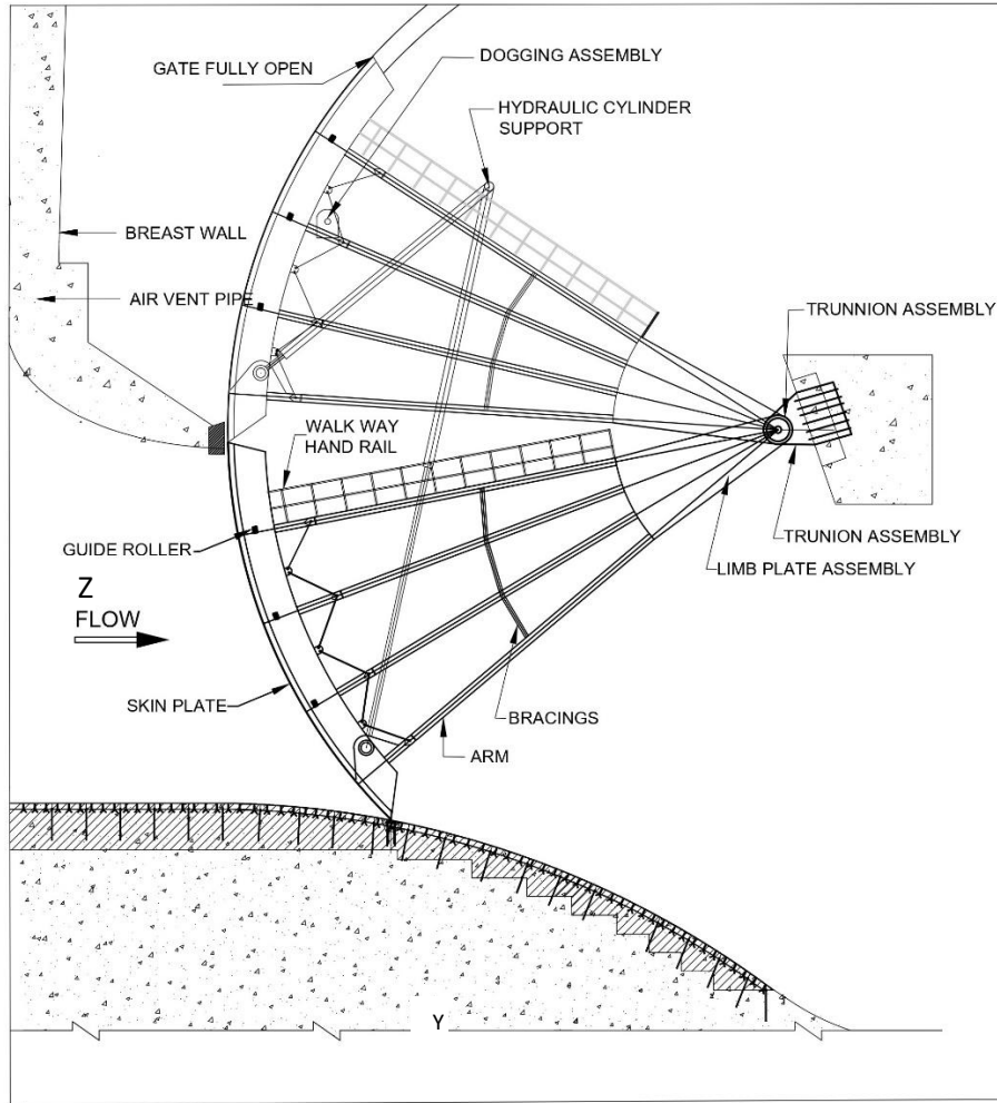
(A) SECTIONAL VIEW OF SLUICE RADIAL GATE
