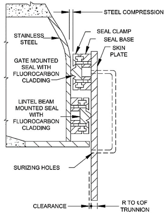
(C) DETAILS OF TOP SEAL
