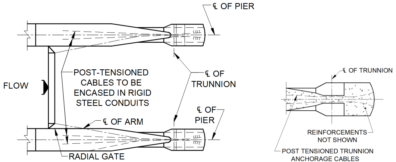
(B) PLAN OF PEIRS SHOWING ANCHORAGER
