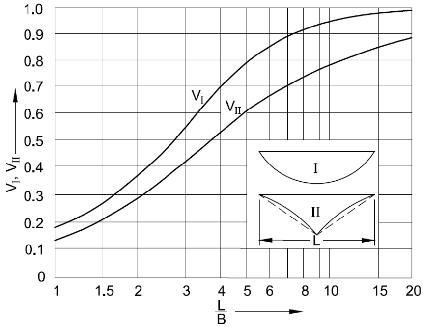
FIG. 13 CURVES SHOWING RELATIONSHIP BETWEEN L/B AND REDUCTION FACTORS V_I AND V_{II}
