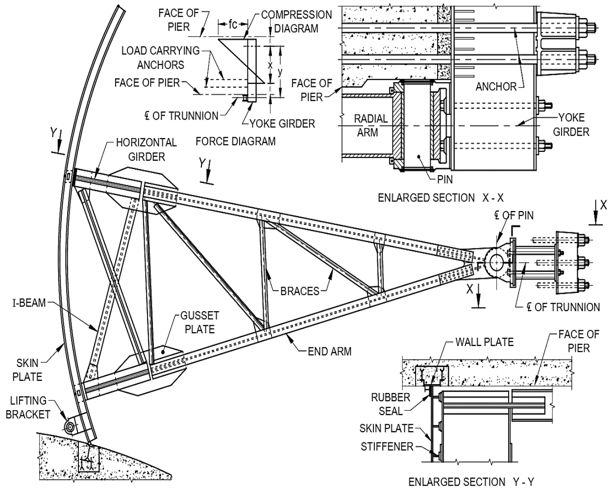
FIG. 1 ILLUSTRATIVE DIAGRAM FOR CREST TYPE RADIAL GATE WITH PARALLEL ARM
