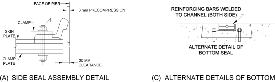
FIG. 2 ILLUSTRATIVE DIAGRAM FOR CREST TYPE RADIAL GATE WITH INCLINED ARM
