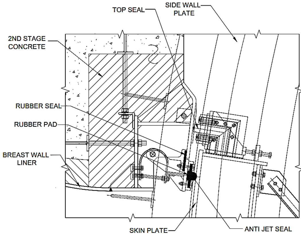
(F) ARRANGEMENT OF TOP SEAL
