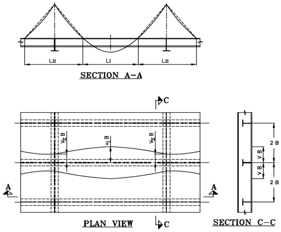
FIG.12 FIGURE SHOWING VARIATION OF CO-ACTING WIDTH FROM SUPPORT TO SUPPORT
