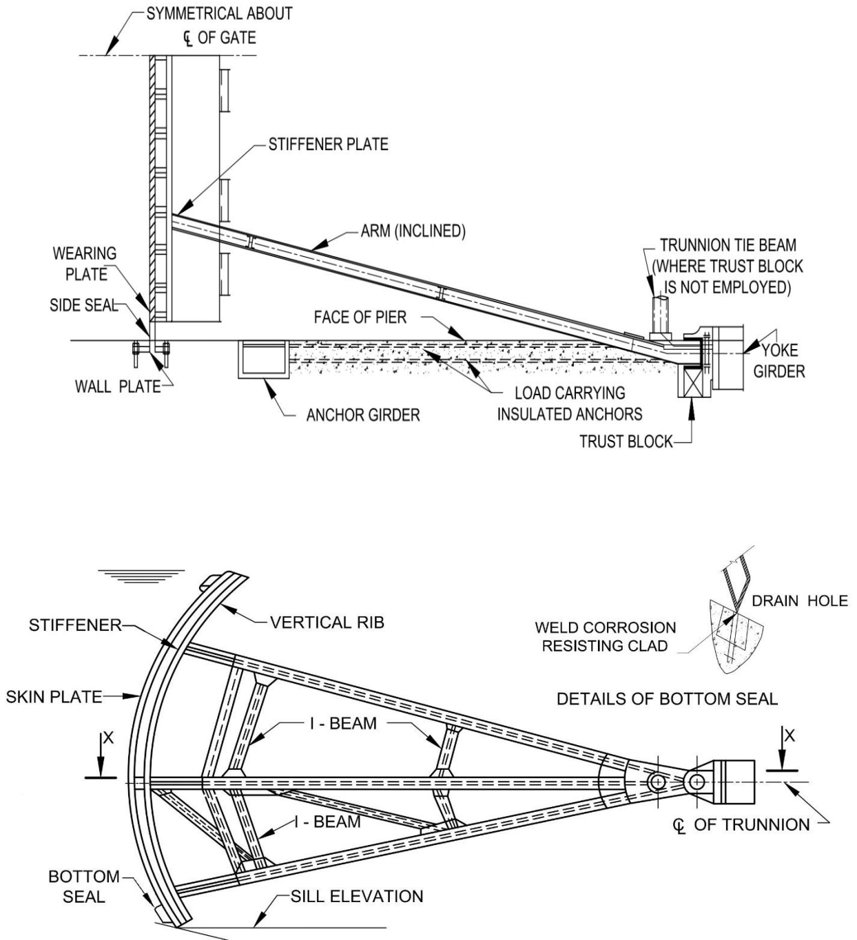
(A) CREST TYPE RADIAL GATE WITH INCLINED ARM
