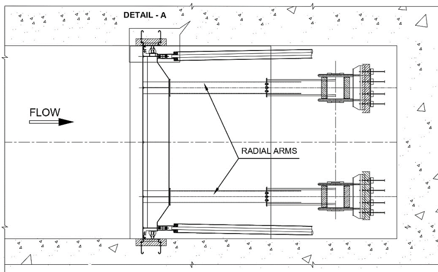
(B) PLAN VIEW OF SLUICE RADIAL GATE
