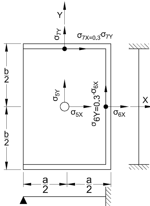
FIG. 8 TWO SHORT AND ONE LONG EDGES FIXED AND ONE LONG EDGE SIMPLY SUPPORTED
