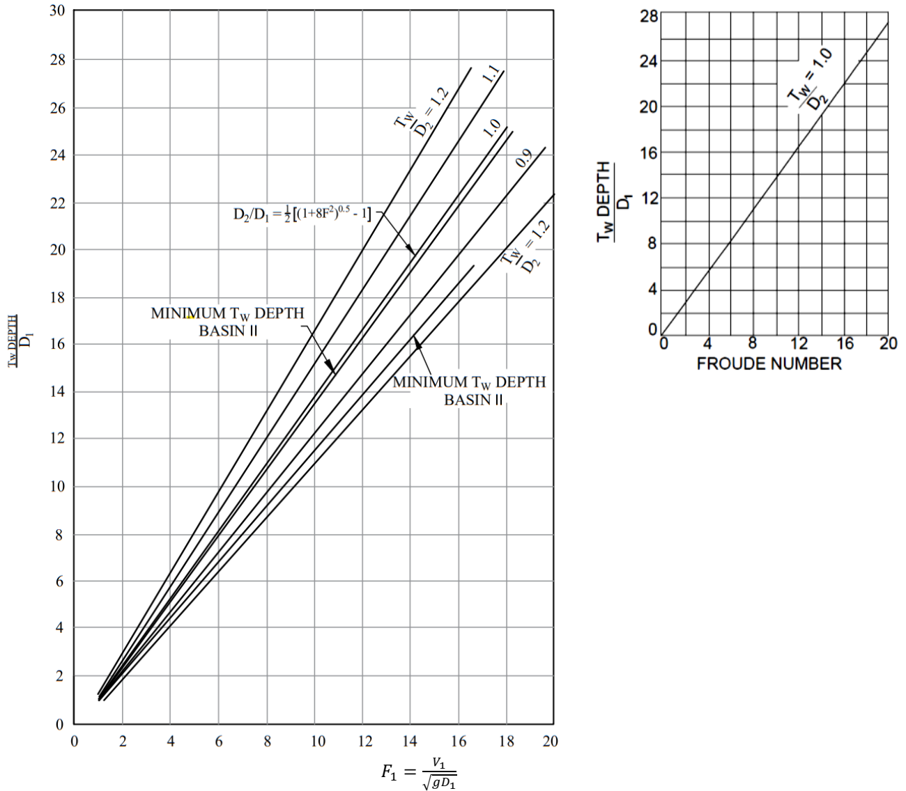
FIG. 9 RATION OF TAIL WATER DEPTH TO D_1 VS FROUDE NUMBER (BASIN I AND II)
