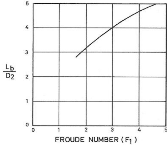
7A RECOMMENDED LENGTH FOR BASIN I
