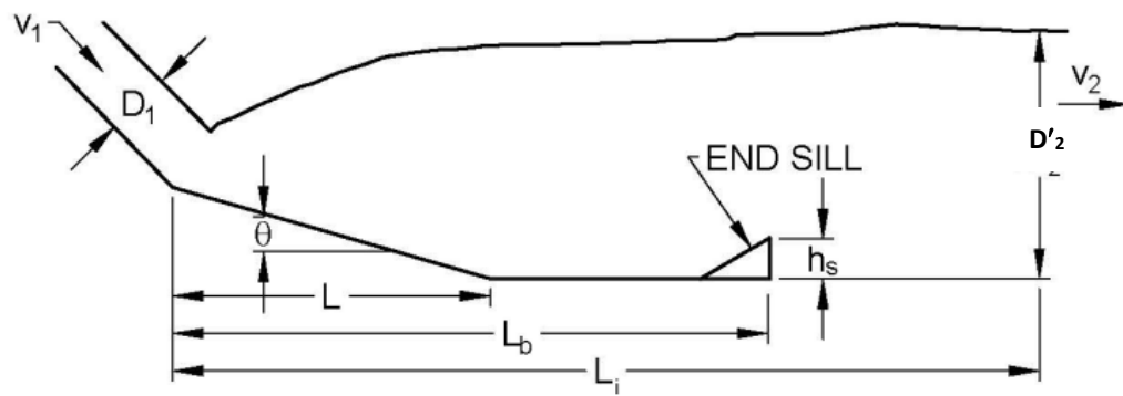
(B) DEFINITION SKETCH BASIN IV
