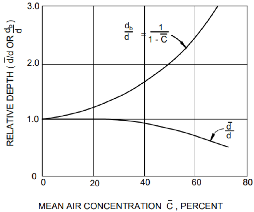
FIG. 14 AIR CONCENTRATION IN FLOW (FALVEY, 1980)
