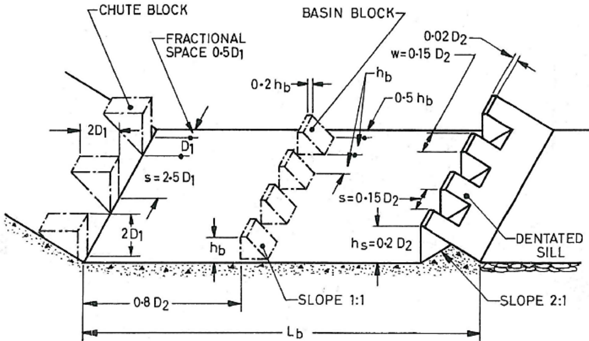
7B APPURTENANCES FOR BASIN I
