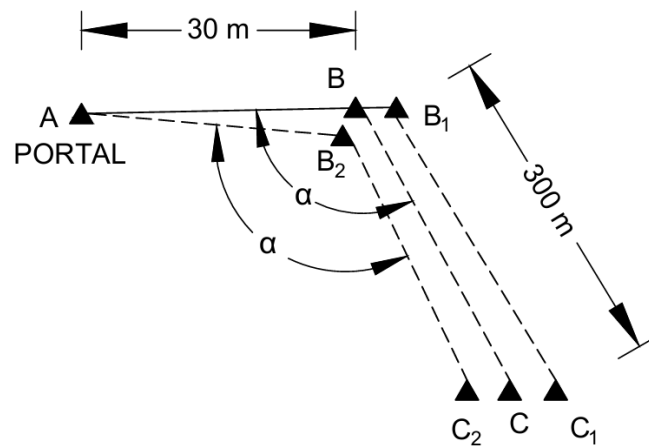
FIG. 7 EFFECTS OF CUMULATIVE ERRORS IN SURVEYING
