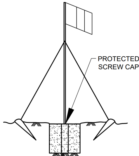
FIG. 5 TYPICAL TARGET
