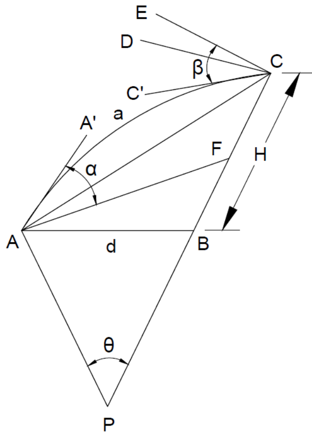
FIG. 8 RECIPROCAL LEVELLING
