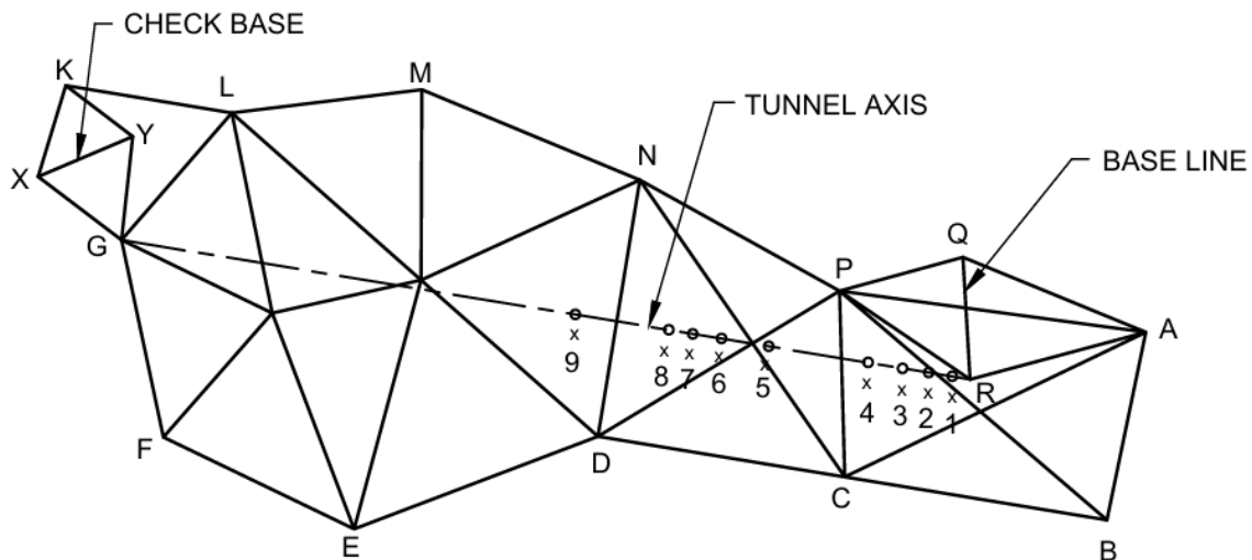
FIG. 3 TYPICAL TRIANGULATION SCHEME
