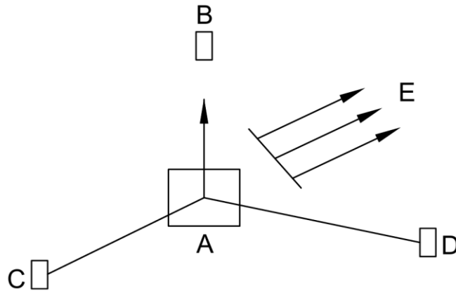
FIG. 9 SETTING OUT OF CENTRELINE OF TUNNEL
