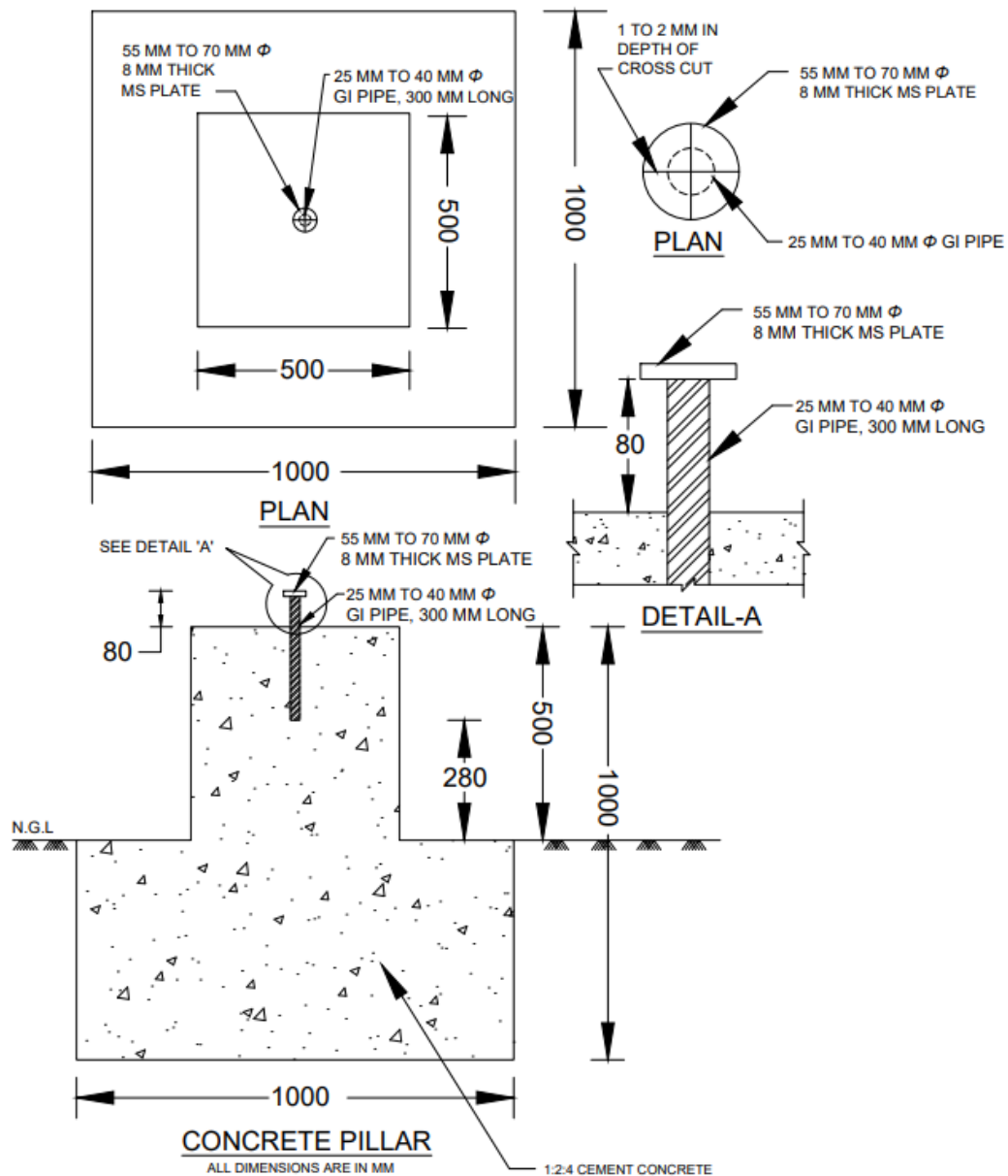
FIG. 1 CONCRETE PILLARS
