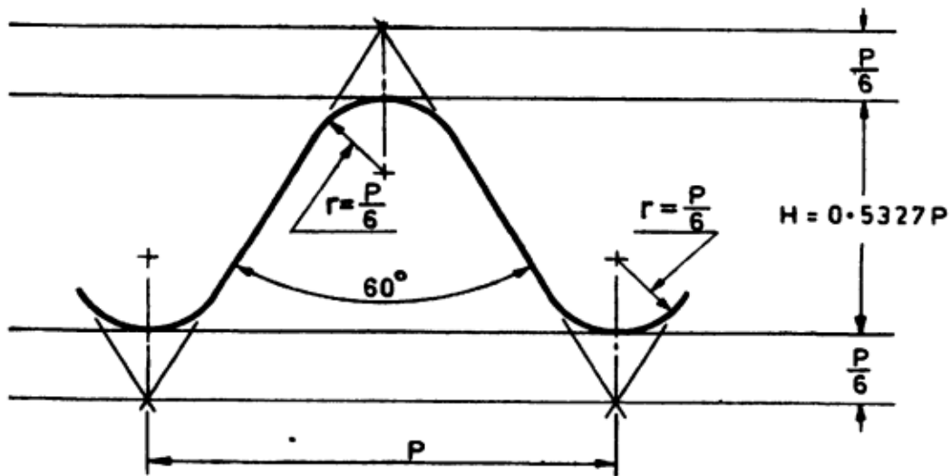
FIG. 2 FORM OF THREAD
