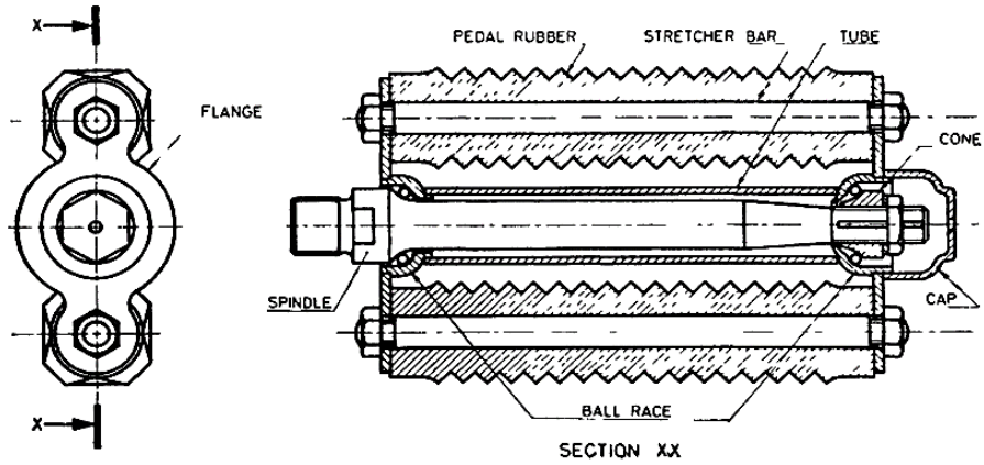
FIG. 3 BLOCK TYPE PEDAL ASSEMBLY (SCHEMATIC)
