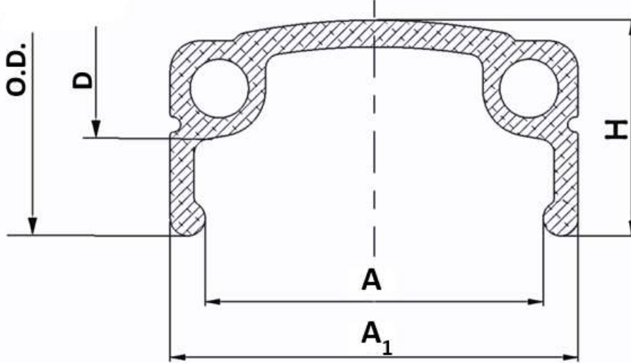
FIG. 22 SINGLE WALL ALLOY RIMS
