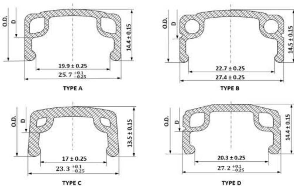
FIG. 8 SINGLE WALL ALLOY RIMS
