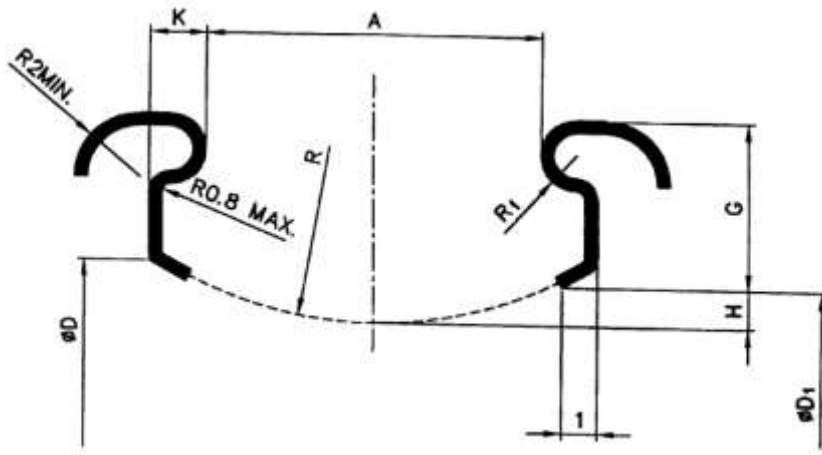
FIG. 19 CROTCHET TYPE RIMS
