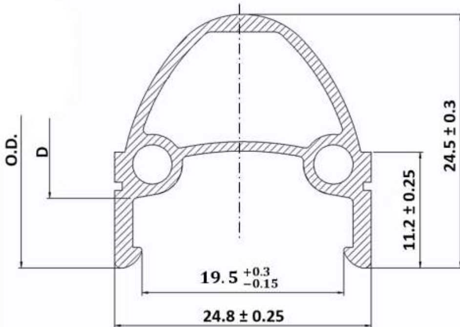
FIG. 9 DOUBLE WALL ALLOY RIM
