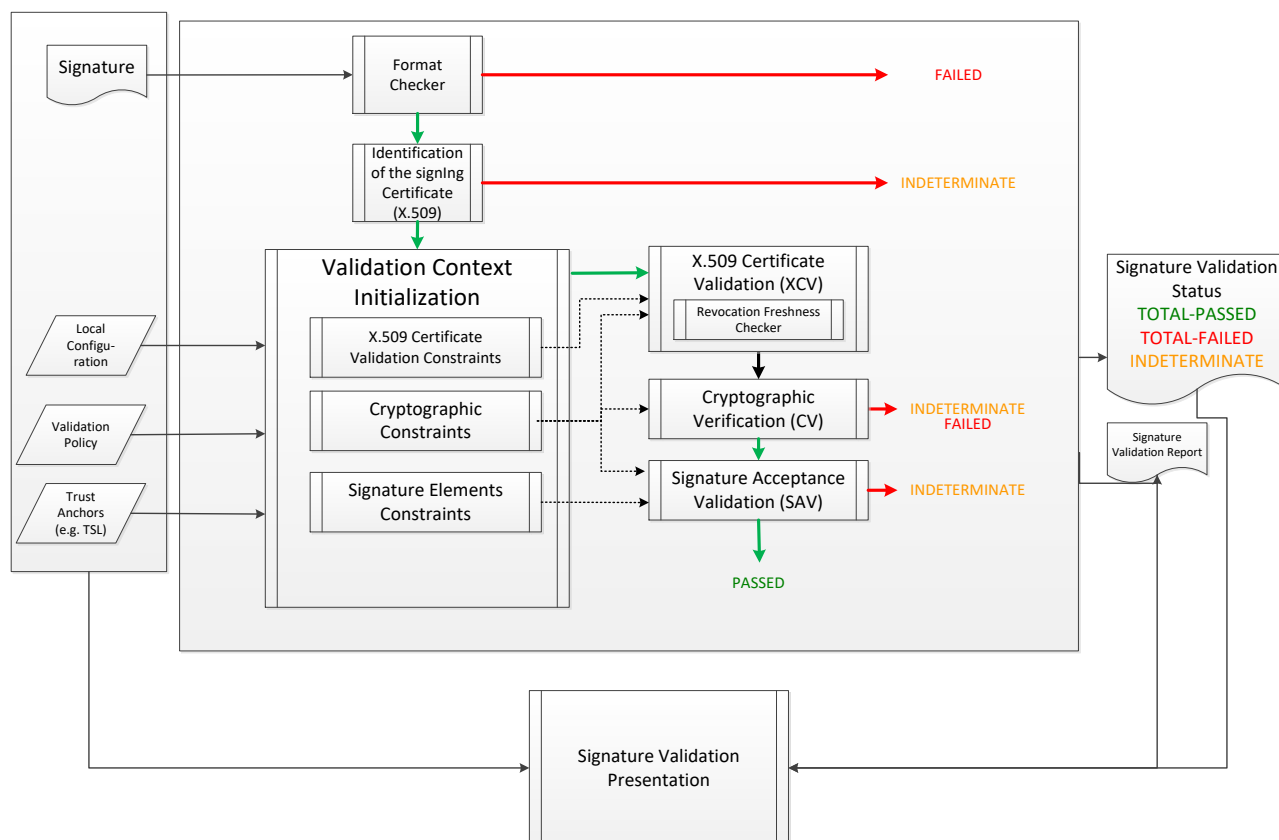
FIG. 12 BASIC SIGNATURE VALIDATION
