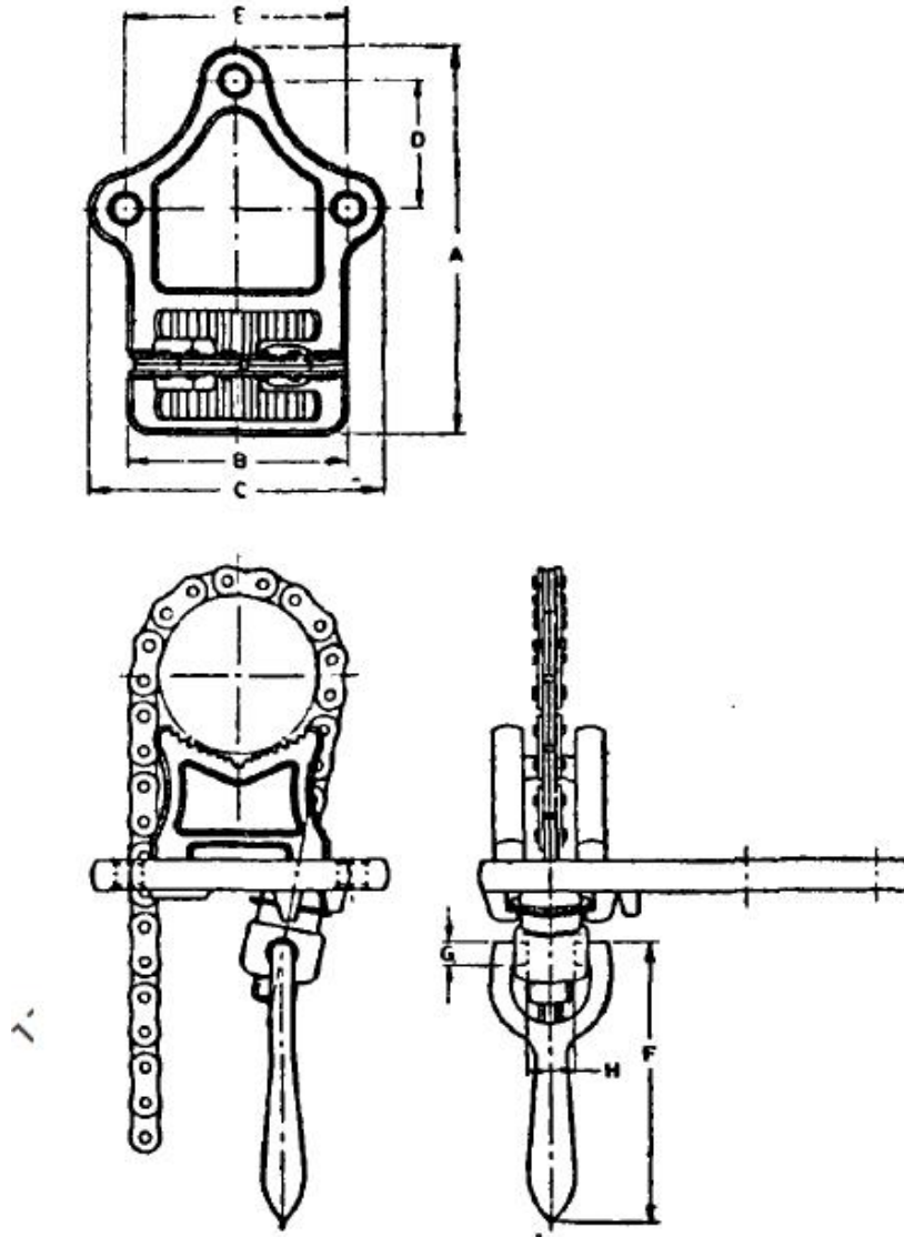
FIG. 1 DIMENSIONS FOR PIPE VICES (CHAIN TYPE)
