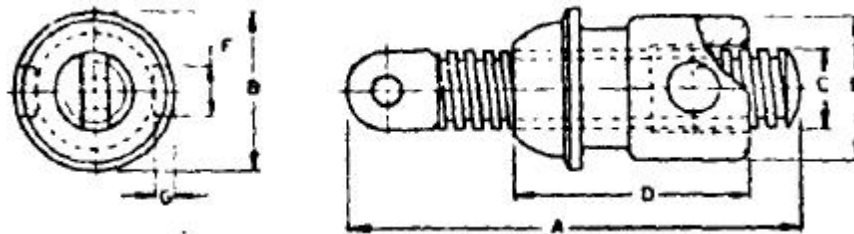
FIG. 3 DIMENSIONS FOR SCREW-NUT ASSEMBLY
