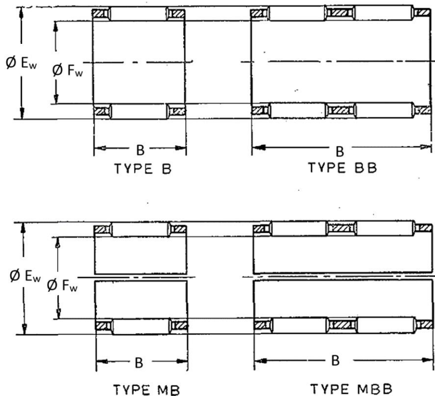
FIG. 1 TYPES OF NEEDLE CAGES
