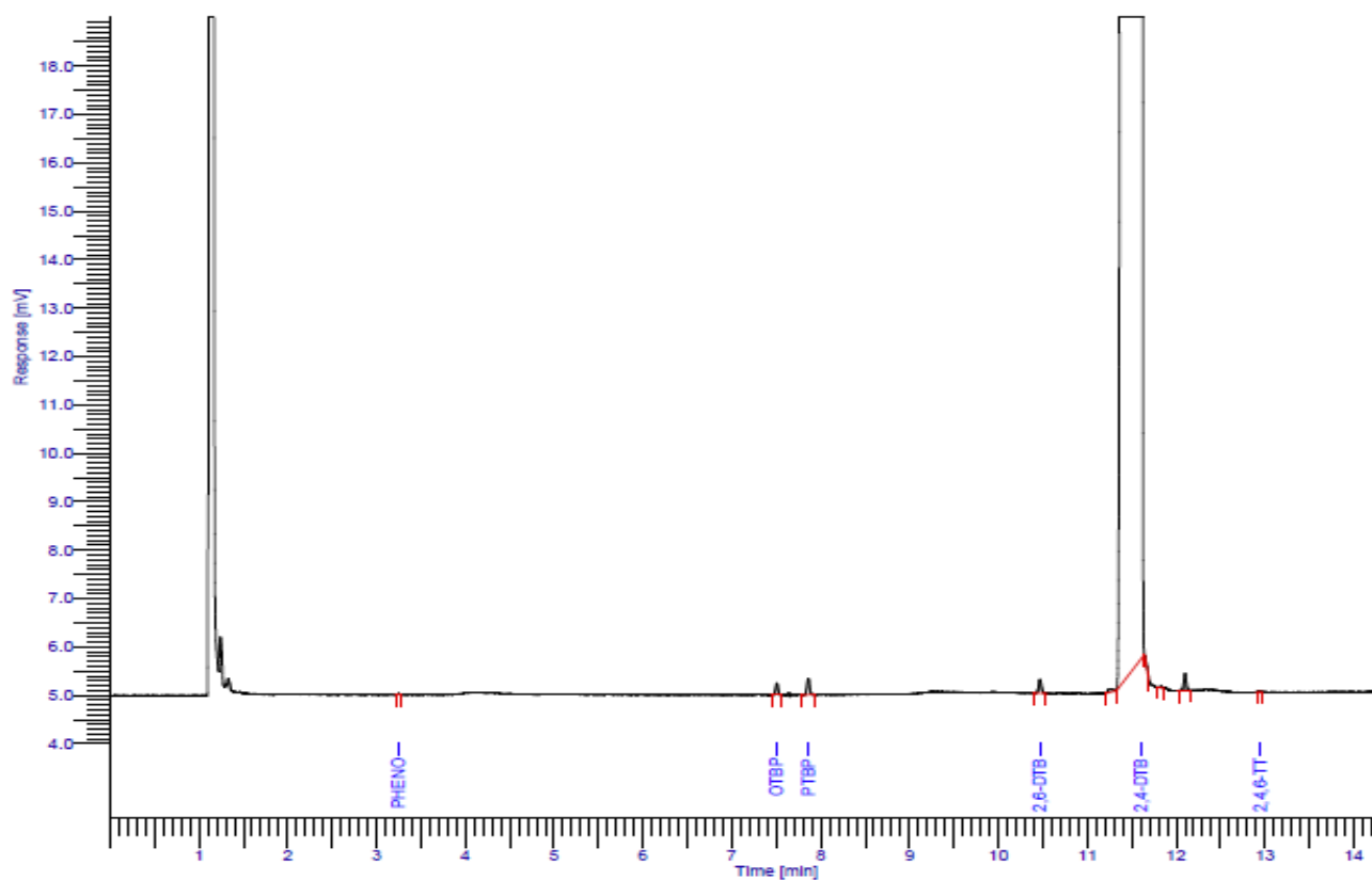
FIG. 1 TYPICAL CHROMATOGRAM
