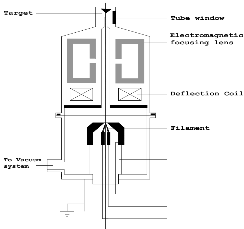
FIG. 3. TYPICAL COMPONENTS IN MICRO-FOCUS X-RAY UNIT.
