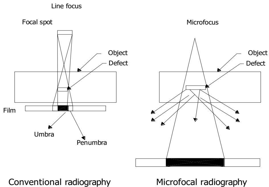
FIG. 1 IMAGE DUE TO POINT SOURCE OF RADIATION AND LINE SOURCE OF RADIATION
