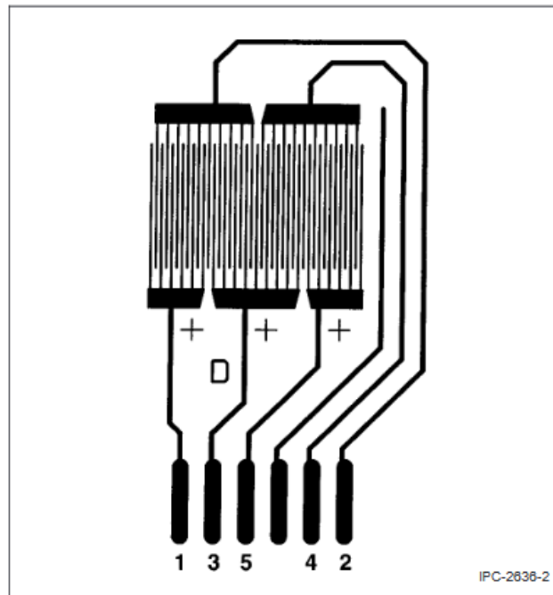
FIG 8 COMB PATTERN BIAS APPLICATION
