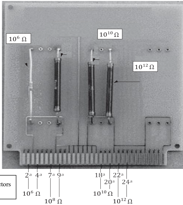
FIGURE 11 RESISTOR VERIFICATION COUPON
