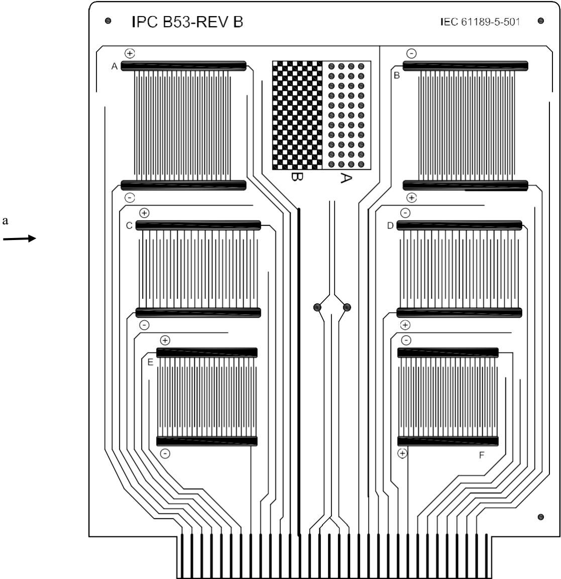
FIG. 13 IPC B53-REV B TEST COUPON LOCATION WITH RESPECT TO CHAMBER AIR FLOW
