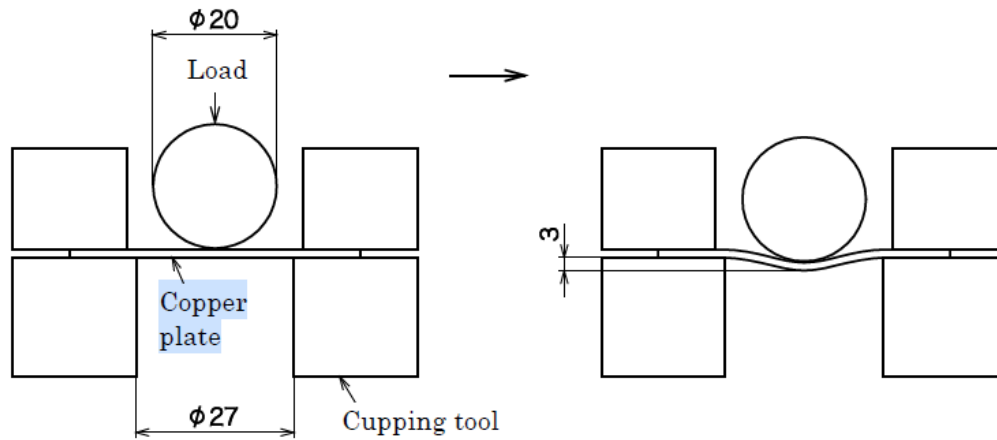
FIG. 2 DIMENSIONS OF PENETRATOR, DIE AND BLANK-HOLDER
