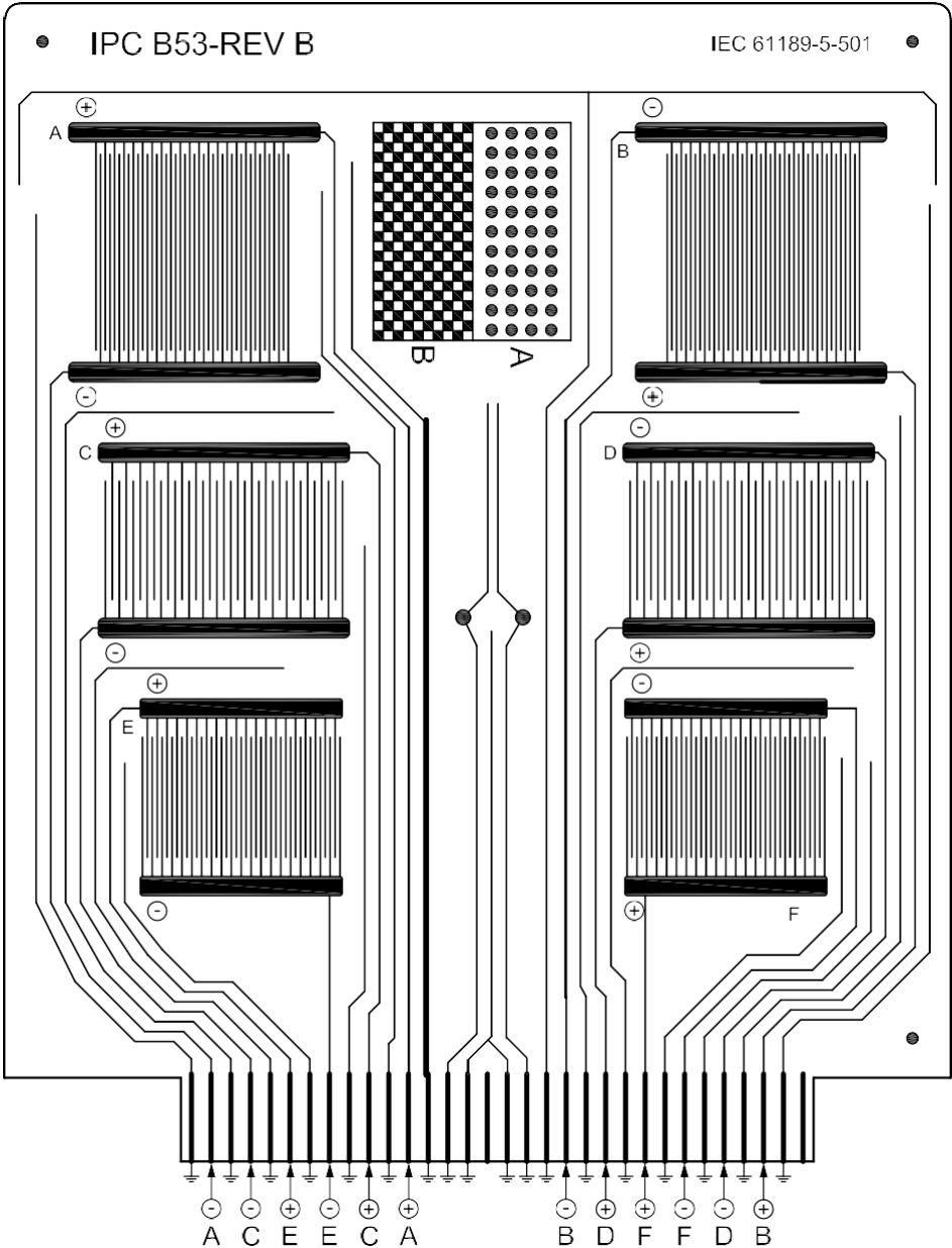
FIG. 14 IPC B53-REV B TEST COUPON CONNECTIONS ACCORDING TO IPC-TM-650
