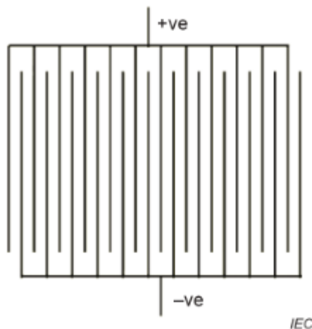
FIG. 9 SIR PATTERN (SOURCE IEC)
