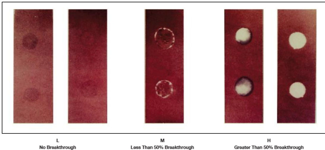
FIG. 1 FLUX TYPE CLASSIFICATION BY CORROSIVITY BY COPPER MIRROR TEST (SOURCE IEC 61189-5-2:2015)
