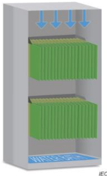
FIG. 7 COUPON ORIENTATION IN TEST CHAMBER (SOURCE IEC)
