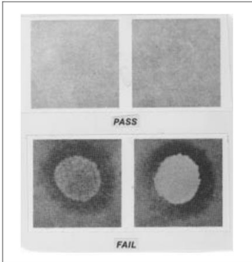
FIG. 4 CHLORIDES AND/OR BROMIDES TEST RESULTS (SOURCE IEC)
