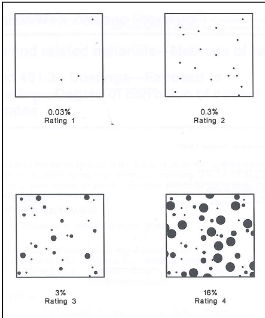
FIG 3. —Typical Corrosion on the Stripped Metal Substrate
