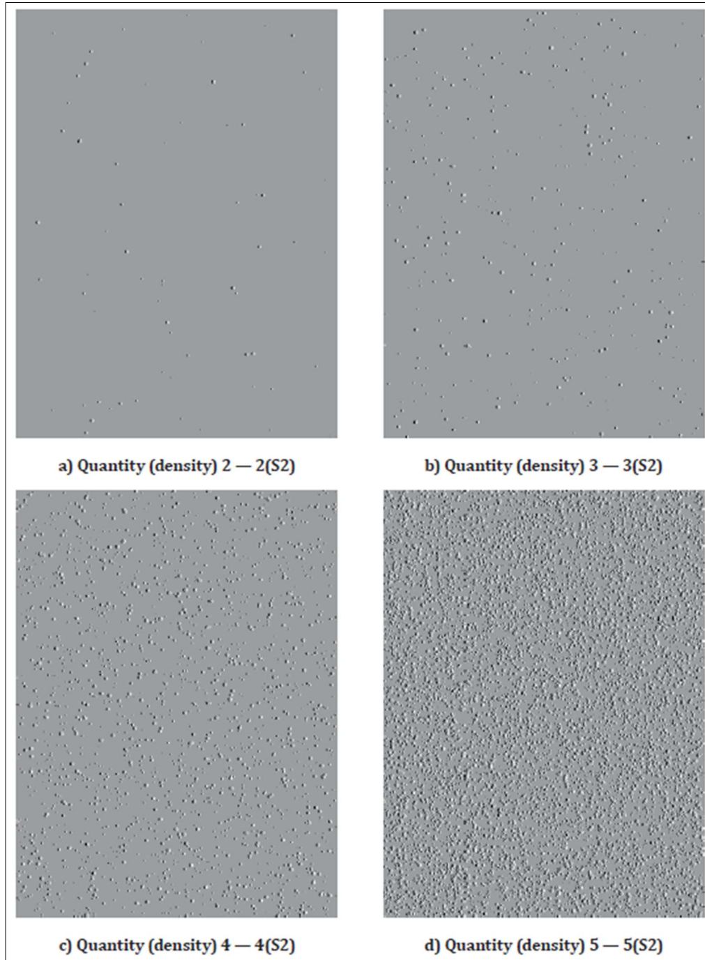
FIG. 4 — Blisters of Size 3
