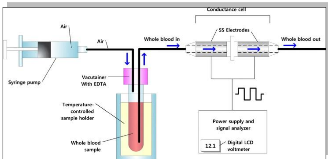
Figure 4: Conductivity method (Clause 4.1)
