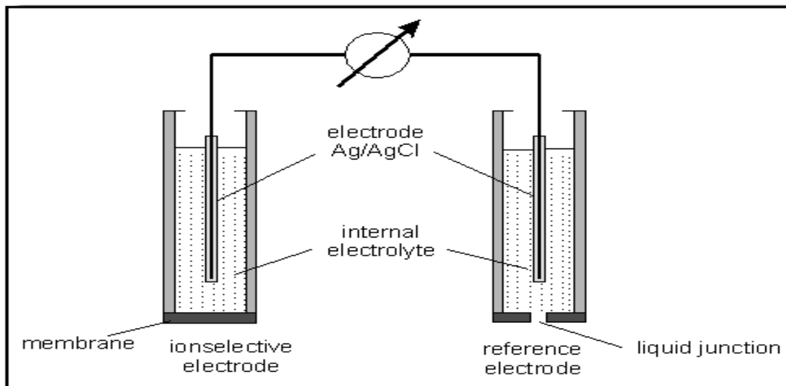
Figure 1: Quantitative, ion selective electrode technology (Clause 4.1)
