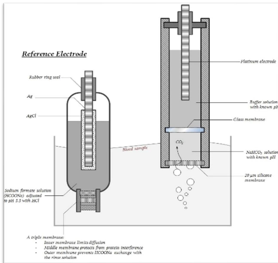
Figure 2: Quantitative: Traditional electrode technology (Clause 4.1)
