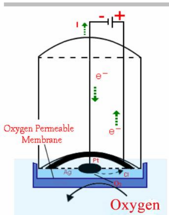
Figure 3: Amperometric technology (Clause 4.1)
