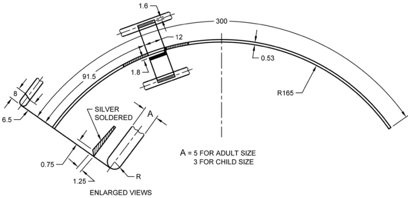
FIG. 1 GUIDE, SAW, DE MARTEL'S PATTERN
