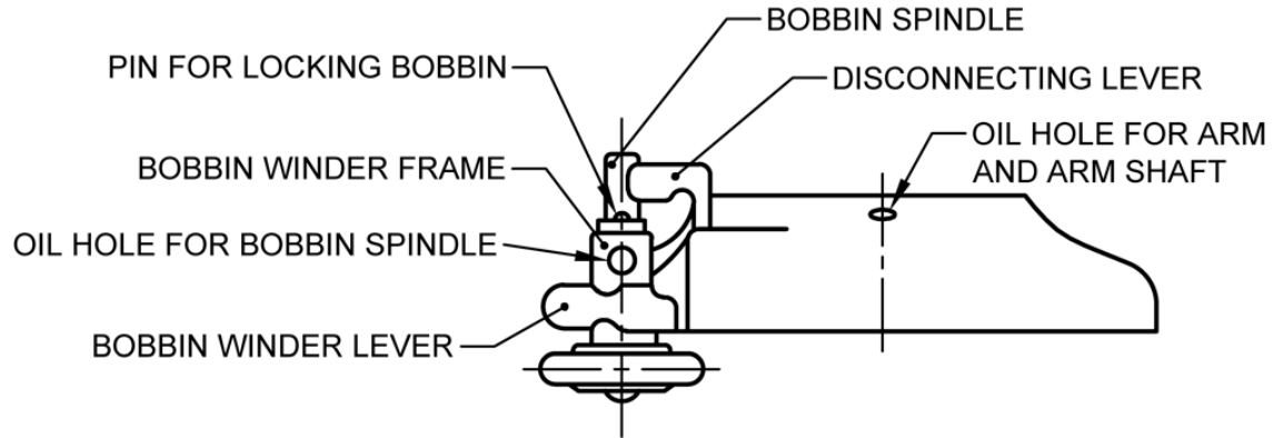
FIG. 1 TERMINOLOGY FOR BOBBIN WINDER ASSEMBLY
