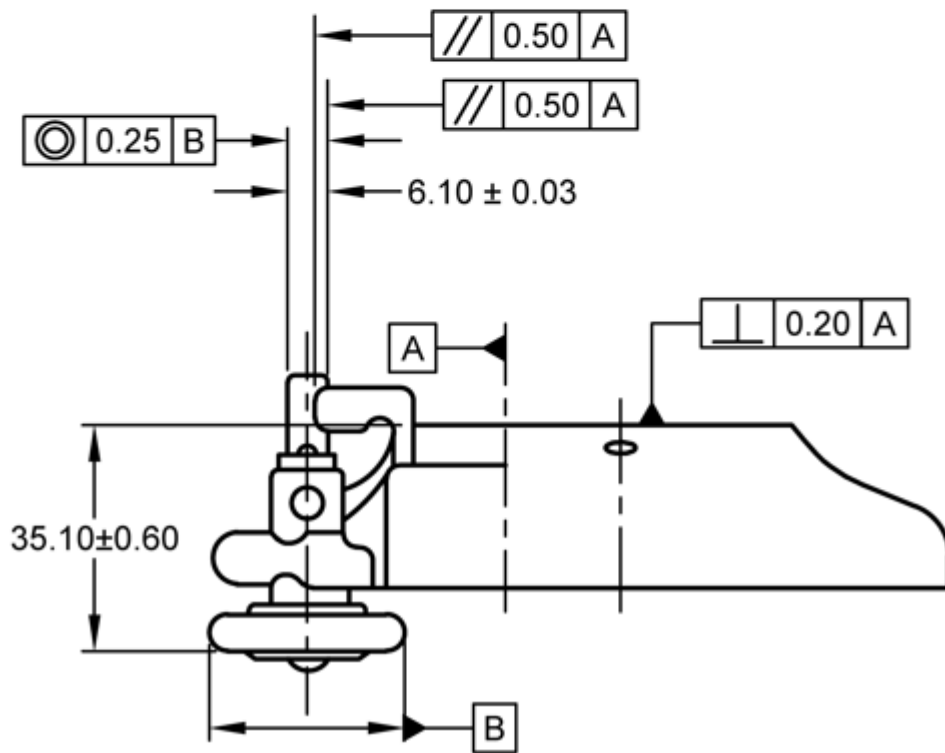
FIG. 2 DIMENSIONS FOR BOBBIN WINDER ASSEMBLY
