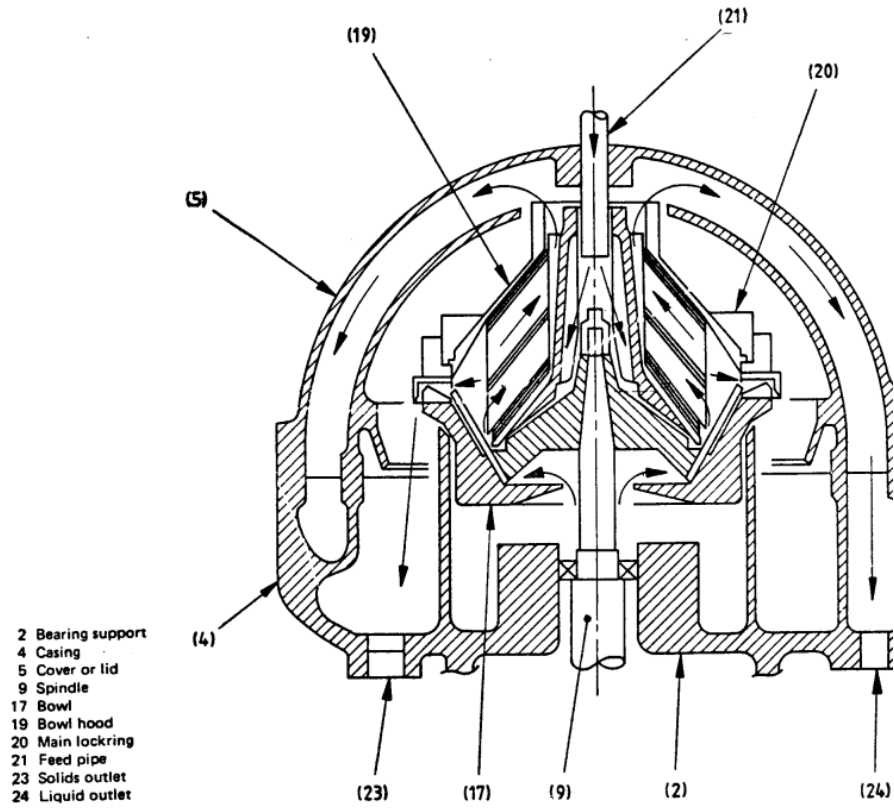
FIG. 13 NOZZLE DISCHARGE DISC CONTINUOUS CENTRIFUGE, SEDIMENTATION MACHINE
