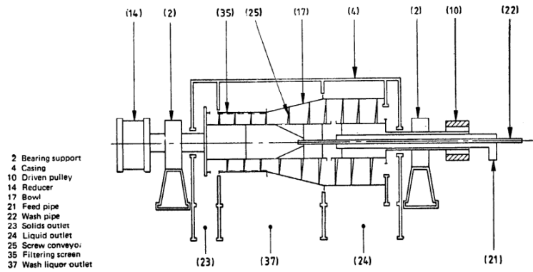
FIG. 16 COMBINED SEDIMENTATION AND FILTRATION MACHINE, SCREEN BOWL DECANTER
