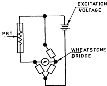
FIG. 3 TWO WIRE ARRANGEMENT FOR PRT SENSOR
