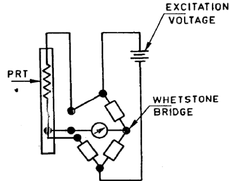
FIG. 4 THREE WIRE ARRANGEMENT FOR PRT SENSOR
