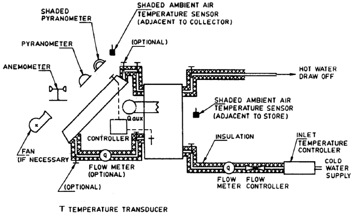
FIG. 2 EXAMPLE OF A TEST LOOP FOR THE MONITORING OF SYSTEM PERFORMANCE
