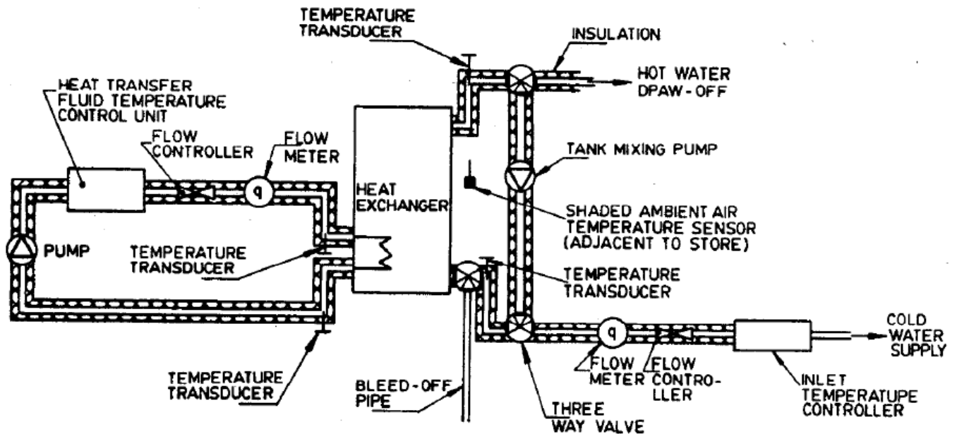
FIG. 1 EXAMPLE OF A STORAGE TESTING FACILITY
