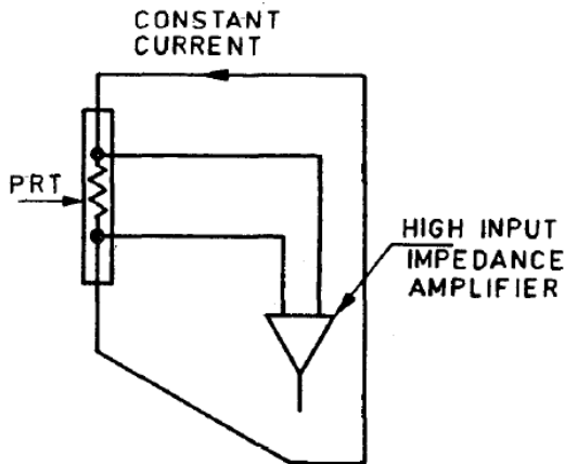
FIG. 5 FOUR WIRE ARRANGEMENT FOR PRT SENSOR
