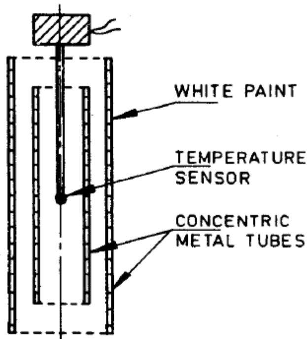
FIG. 11 AMBIENT AIR TEMPERATURE SENSOR
