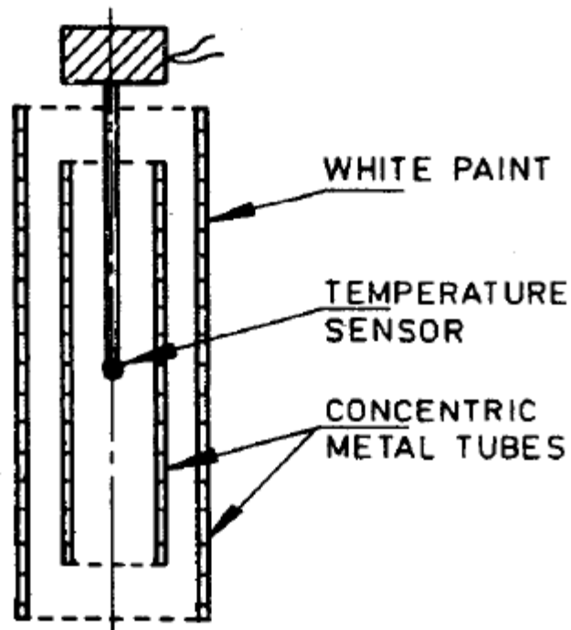
FIG. 11 AMBIENT AIR TEMPERATURE SENSOR
