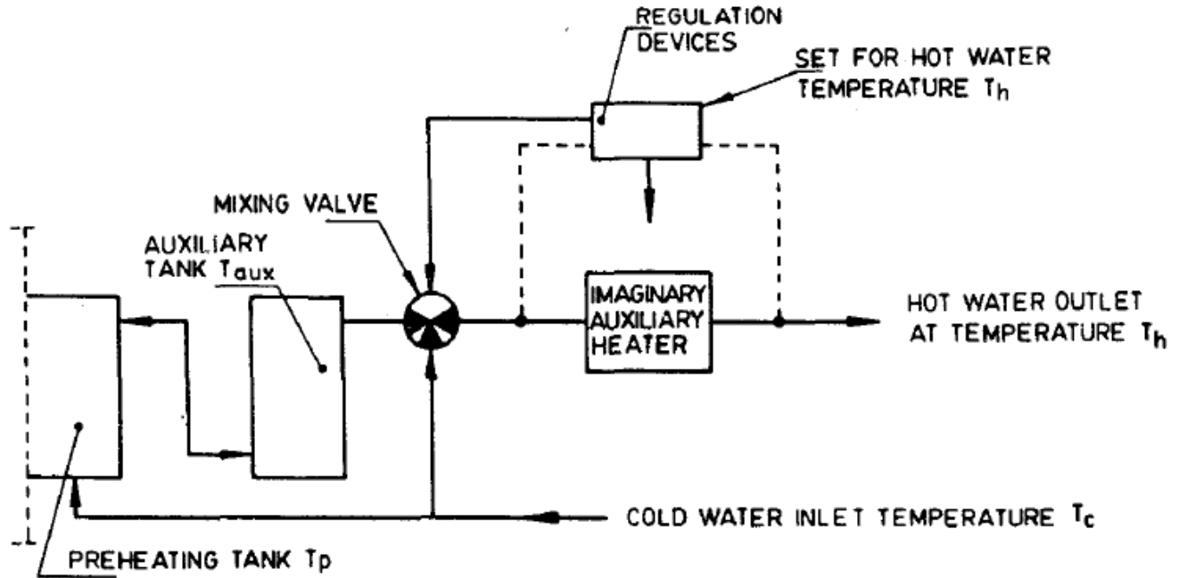
FIG. 15 HOT WATER DRAW-OFF SUBSYSTEM WITH AN AUXILIARY HEATED TANK
