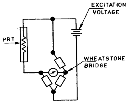
FIG. 3 A TWO WIRE ARRANGEMENT FOR PRT SENSOR
