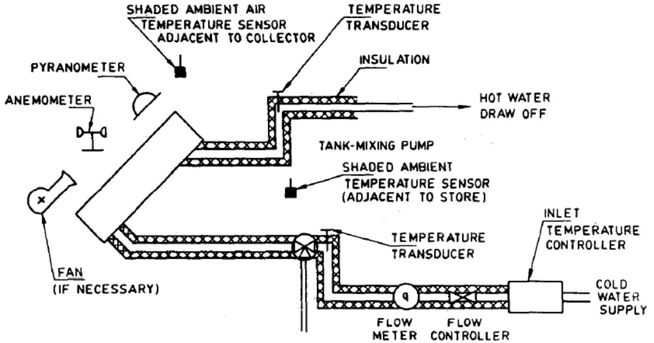
FIG. 12 TEST LOOP FOR THE FORCED/THERMOSIPHON SYSTEM TEST
