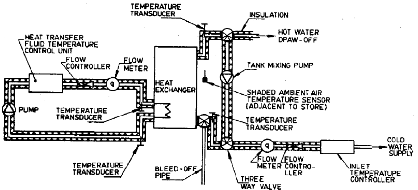
FIG. 1 AN EXAMPLE OF A STORAGE TESTING FACILITY
