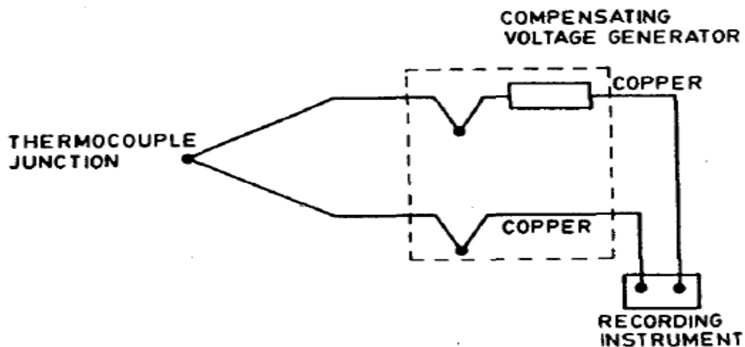
FIG. 7 ARRANGEMENT FOR THERMAL COMPENSATION OF THE JUNCTION BETWEEN THE RECORDING INSTRUMENT AND THERMOCOUPLE
