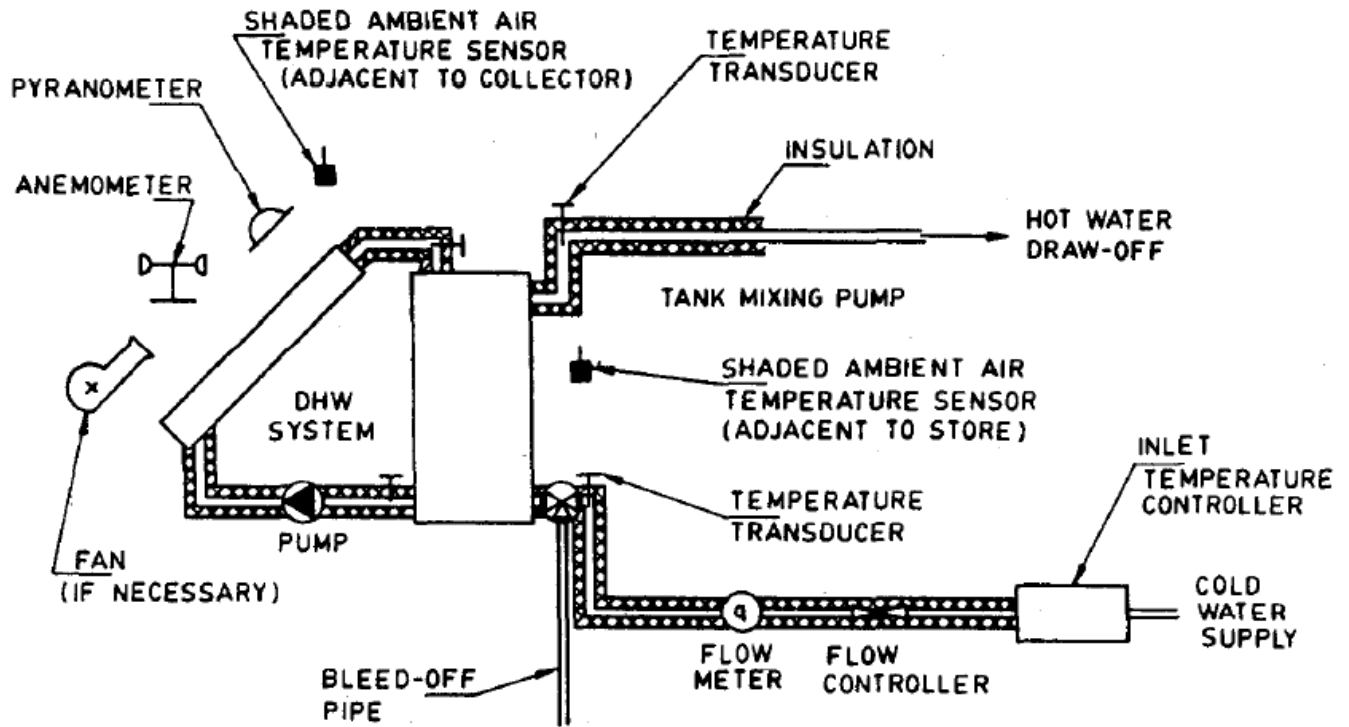
FIG. 13 TEST LOOP FOR THE ICS SYSTEM TEST
