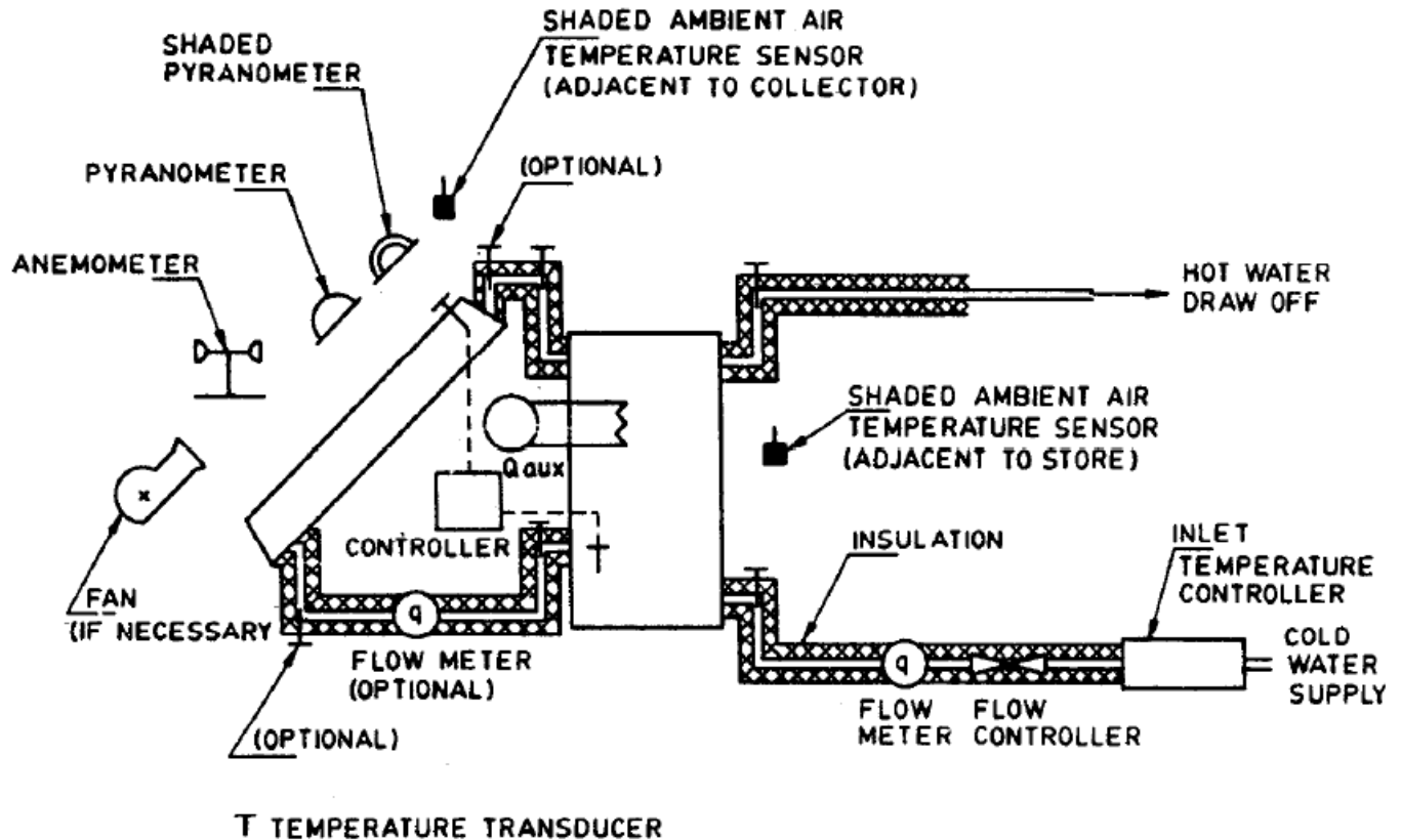
FIG. 2 AN EXAMPLE OF A TEST LOOP FOR THE MONITORING OF SYSTEM PERFORMANCE
