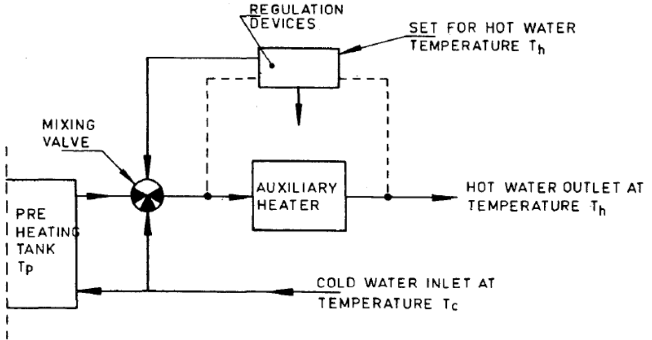
FIG. 14 HOT WATER DRAW-OFF SUBSYSTEM WITH AN AUXILIARY HEATER CONNECTED IN SERIES
