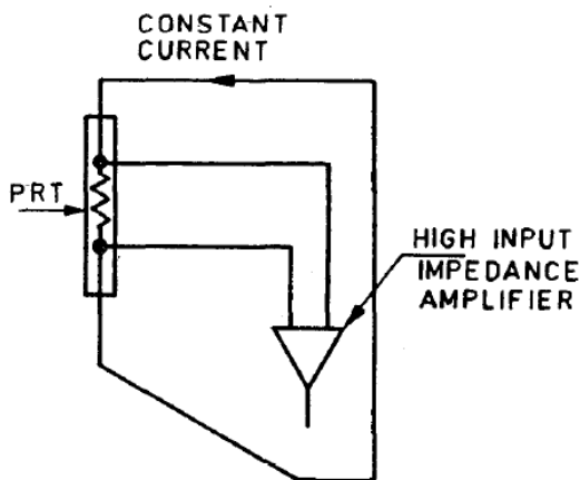
FIG. 5 A FOUR WIRE ARRANGEMENT FOR PRT SENSOR
