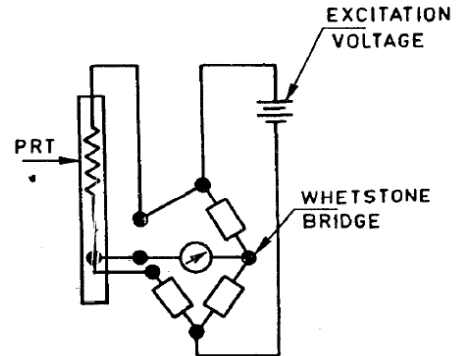
FIG. 4 A THREE WIRE ARRANGEMENT FOR PRT SENSOR
