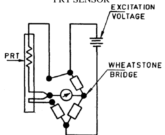
FIG. 6 A FOUR WIRE COMPENSATED ARRANGEMENT FOR PRT SENSOR
