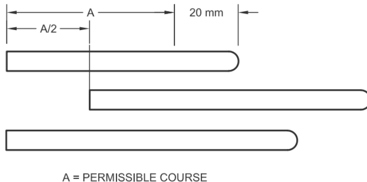
FIG. 7 TEST POSITION FOR SLIDING COMPONENTS WHICH HAVE NO LIMITING STOP
