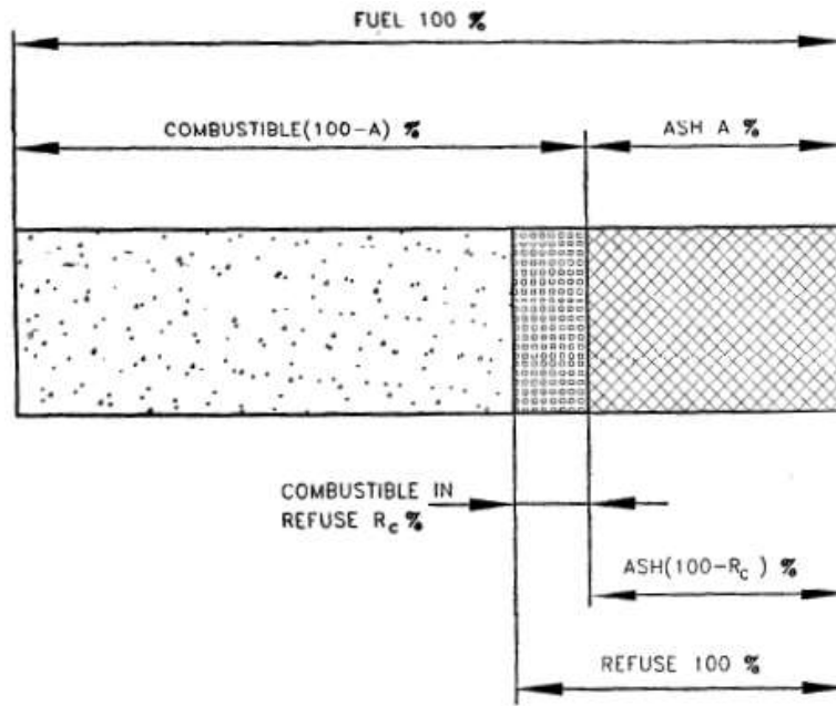
FIG. 1 COMPOSITION OF FUEL
