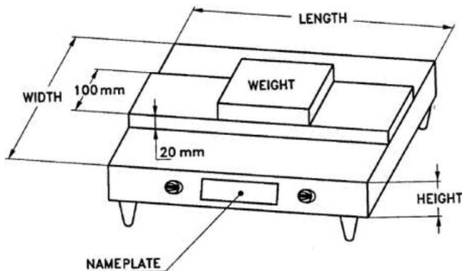
FIG. 2 STRENGTH TEST
