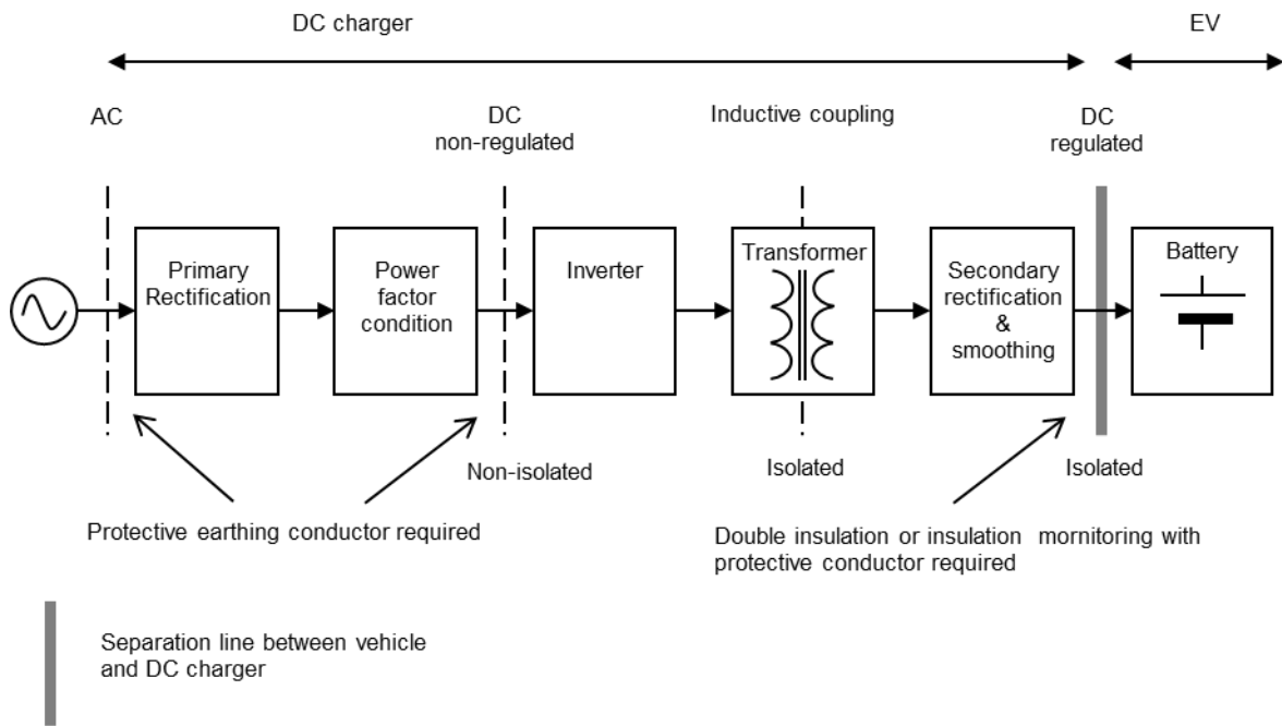
FIG. 39 EXAMPLE OF TYPICAL ISOLATED SYSTEM
