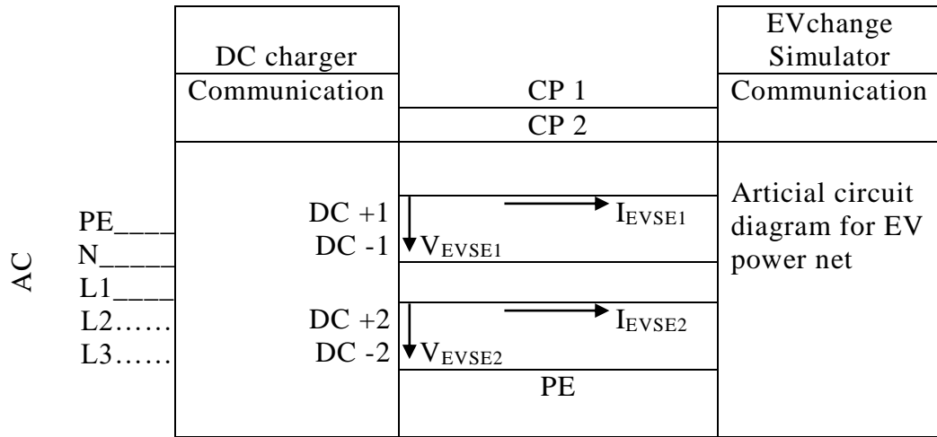
FIG. 31 STANDARD TEST SETUP CIRCUIT DIAGRAM
