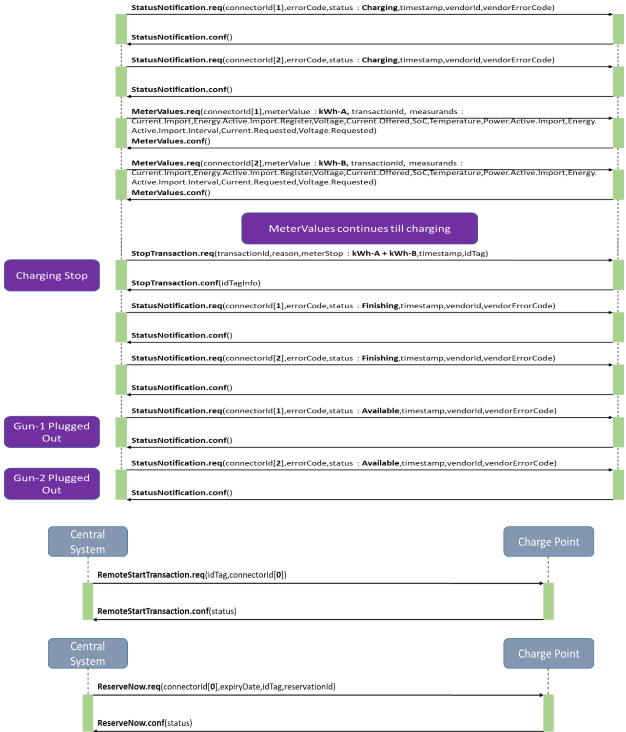
FIG. 46 - COMMUNICATION PROTOCOL BETWEEN EVSE AND CMS
