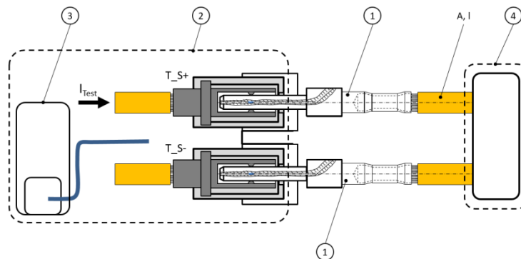
FIG. 13 REFERENCE DEVICE C_0
