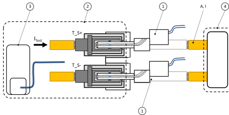
FIG. 15 REFERENCE DEVICE C_1
