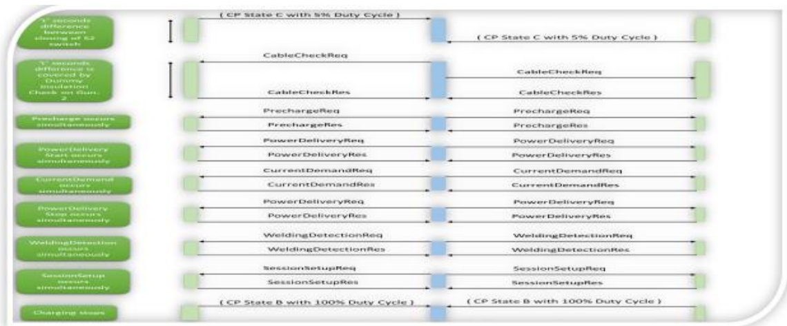
FIG. 21 SEQUENCE DIAGRAM FOR NORMAL START UP
