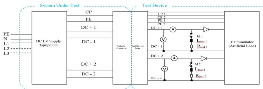
FIG. 38– EV CHARGING AND DISCHARGING MODES
