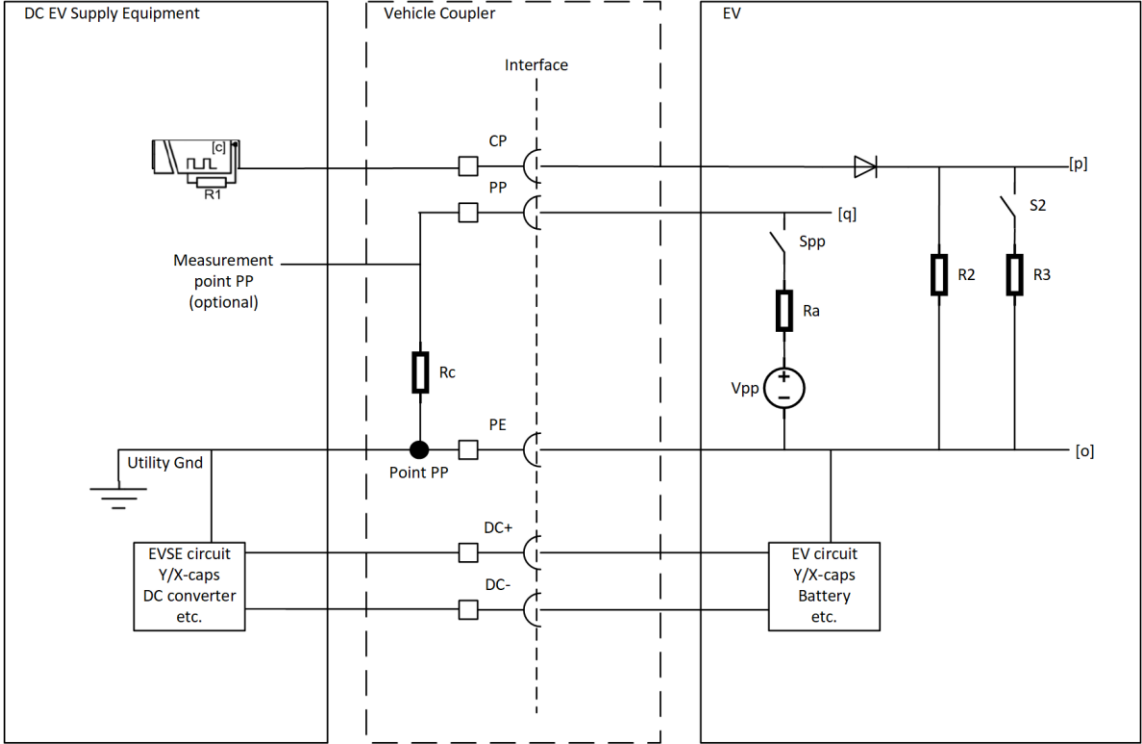
FIG. 19 INTERFACE COMPONENTS FOR CONFIGURATION FF
