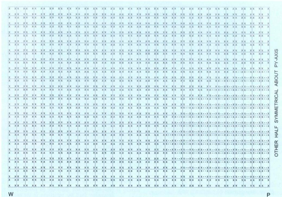
Fig. 6 Lux-Grid I for Daylighting of a Side-lit Window in Absence of External Obstruction
