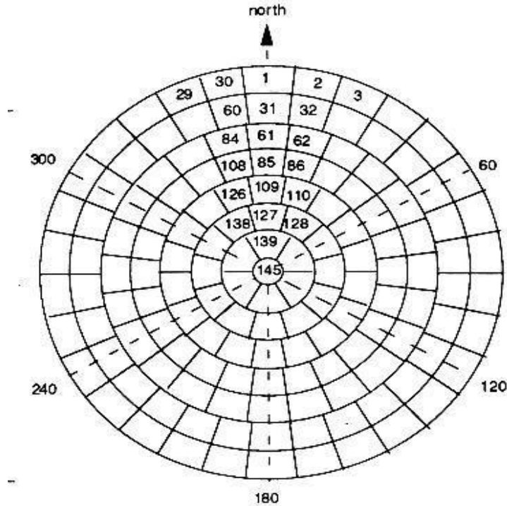
Fig. 3 Sub Division of Sky Vault
