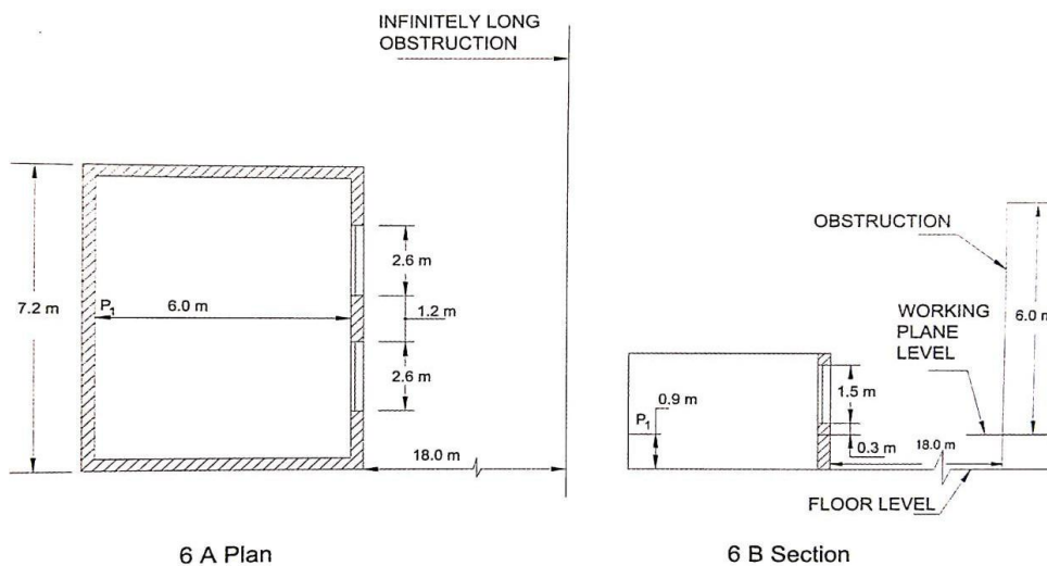
Fig. 8 Typical Example for Windows with External Obstruction
