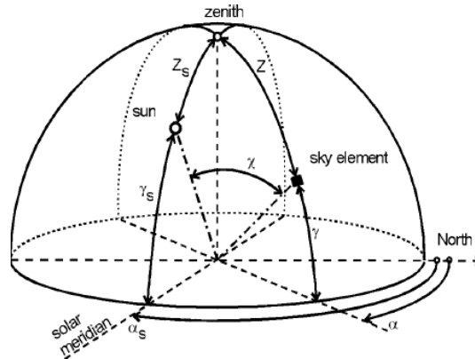
Fig. 2 Angles Defining the Position of the Sun and a Sky Element
