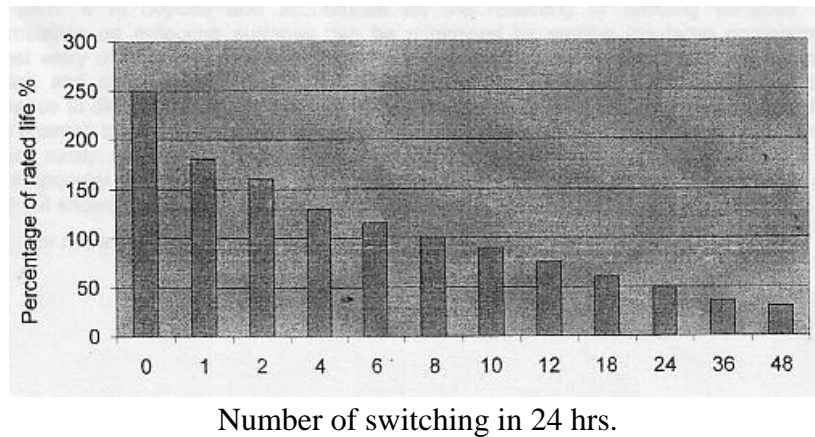
Fig. 3 Example of the Effect of Switching on Lamp Life for Fluorescent Lamp on Lagging Switch Start Circuit
