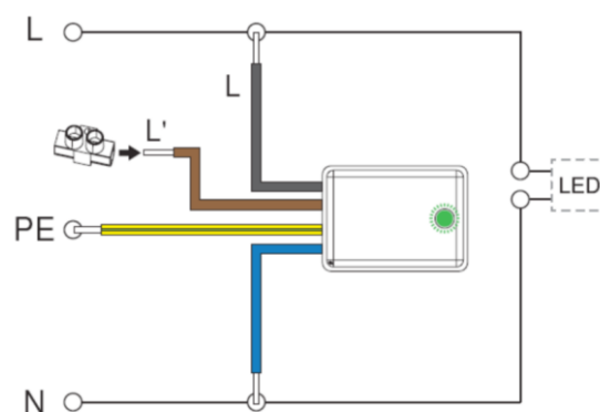
Fig. 1 Parallel Connection
