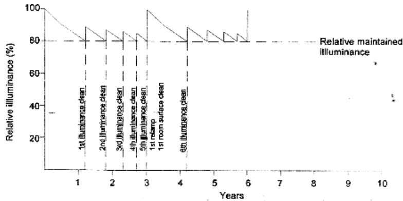
Fig. 6 Variable Interval Maintenance Program
