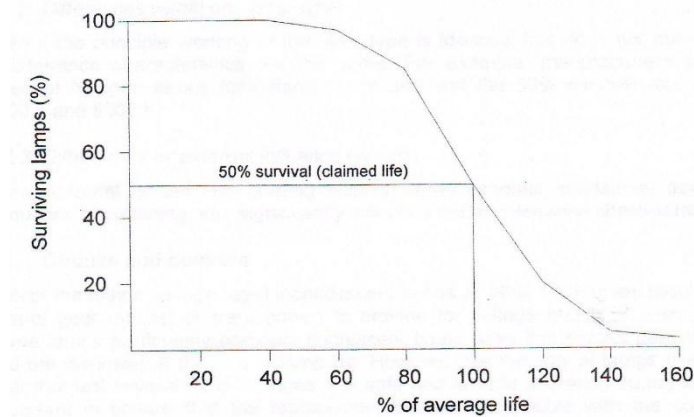
Fig. 2 Typical Lamp Mortality Curves
