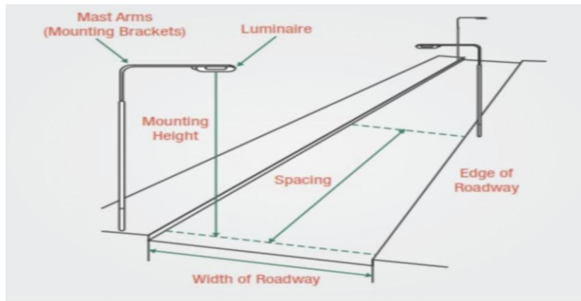
Fig. 3 Street Lighting Geometry
