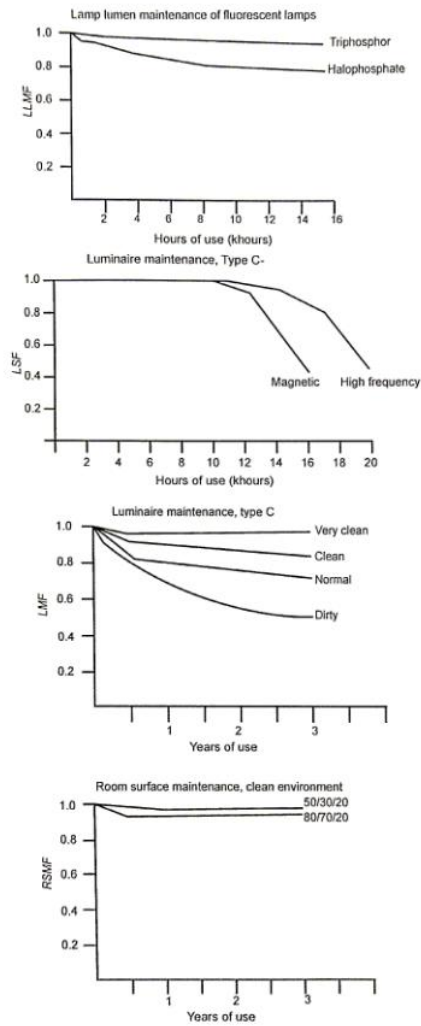
Fig. 4 Examples of Recoverable Maintenance Factor Data
