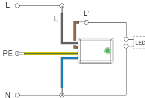
Fig. 2 Series Connection
