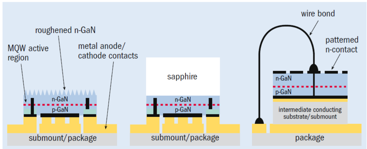
a) Thin-film flip-chip LED chip LED
