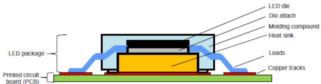
a) Surface Mounted LED Package with Lead Wires
