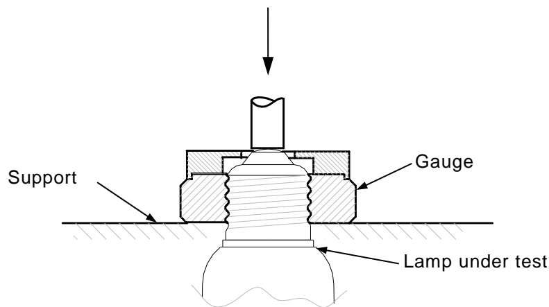
Fig. 6 Test Equipment for Applying an Axial Force
