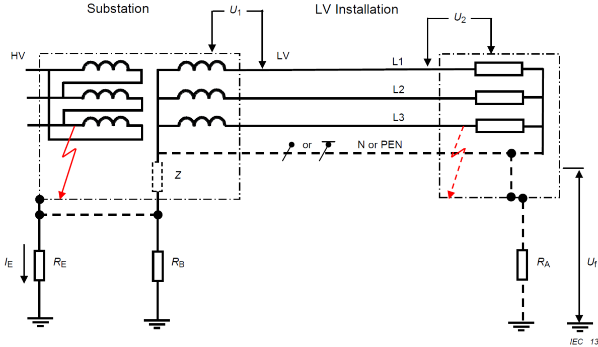
Figure B1 – Representative schematic sketch for possible connections to earth in substation and LV-installation and occurring over-voltages in case of faults
