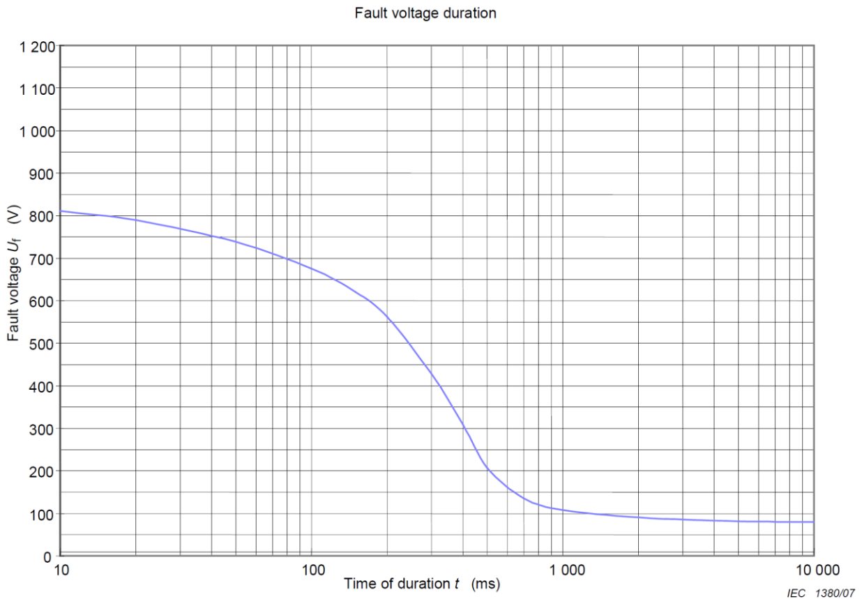
Fig. B2 Tolerable Fault Voltage Due to an Earth-Fault in The HV System
