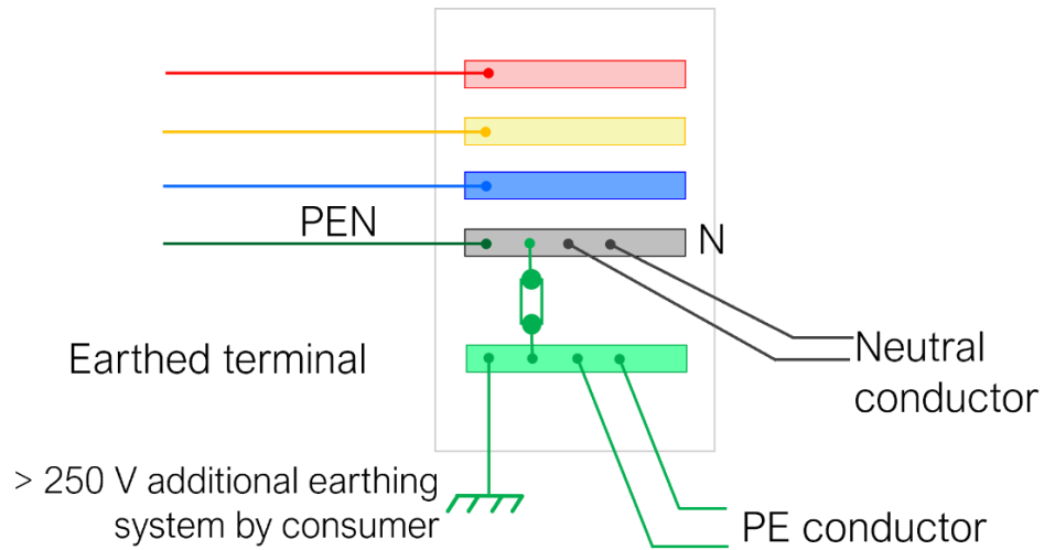
Fig. 12 Typical Connection Diagram of a PEN Conductor in a TN-C-S Network and Separation of PE Conductor Through A Link (Case 2).
