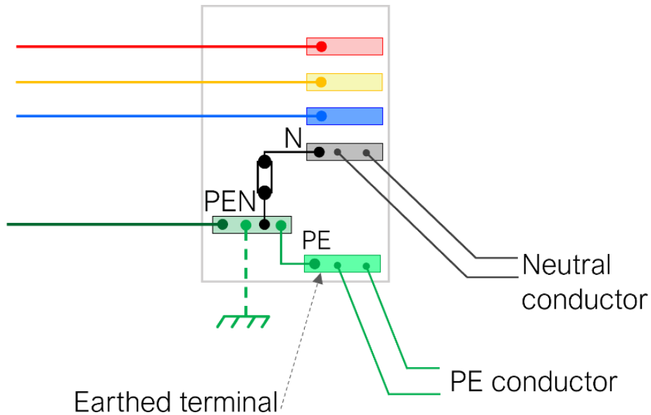
Fig. 13 Typical Connection Diagram of a PEN Conductor in a TN-C-S Network and Separation of PE Conductor Through a Link (Case 3).
