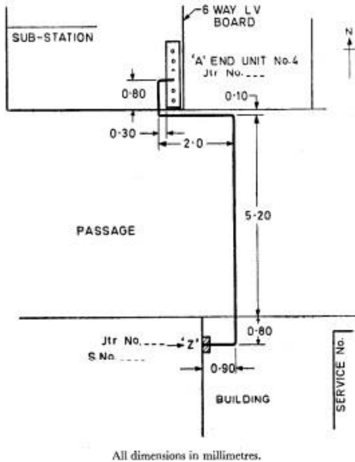
Fig. 16 Typical Diagram Showing Service Line Connected to A Low Voltage Distribution Board of A Sub-Station.
