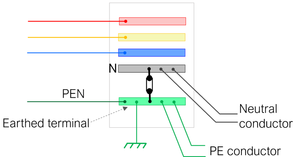
Fig. 11 Typical Connection Diagram of a PEN Conductor in a TN-C-S Network and Separation of PE Conductor Through a Link (Case 1).
