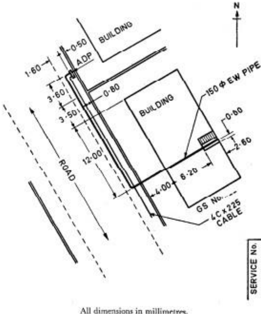
Fig. 15 Typical Diagram Showing Service Line Connected to a Distribution Pillar
