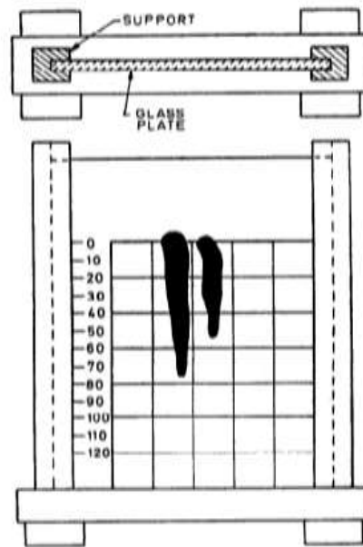
FIG. 1 FLOW GAUGE
