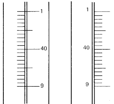
FIG. 4 EXAMPLES OF POSITIONING OF SCALE LINES AND FIGURING FOR SOLID-STEM THERMOMETERS
