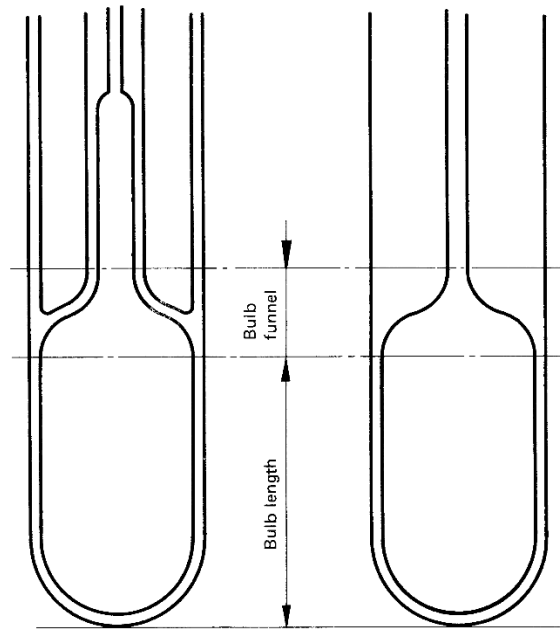
FIG 3 DEFINITION OF BULB LENGTH
