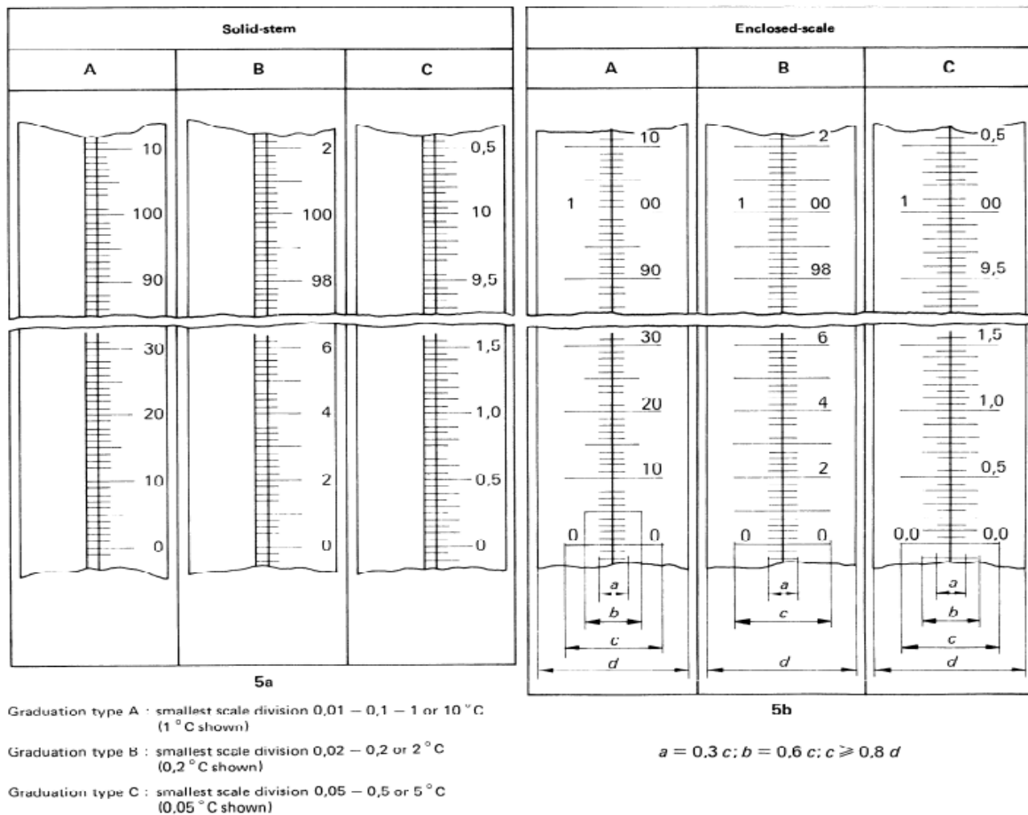
FIG. 5 EXAMPLES OF SCALE LINES AND FIGURING
