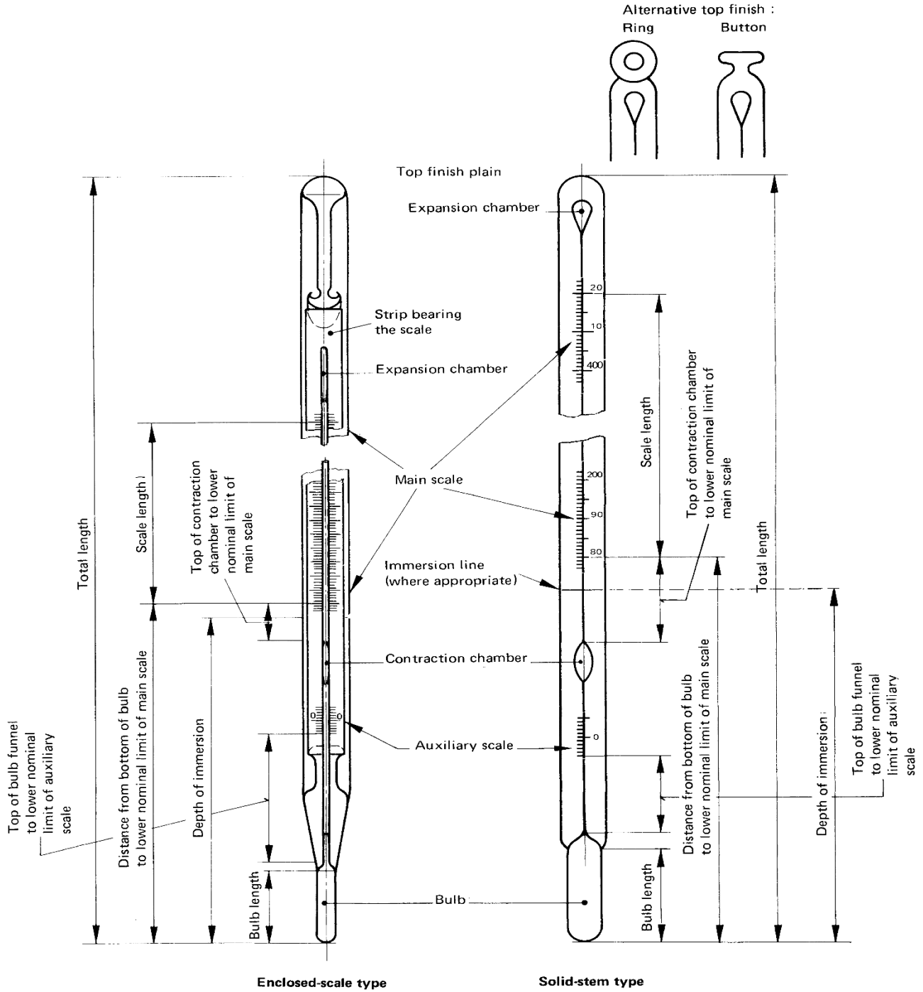
FIG. 1 GENERAL DESIGN AND TERMINOLOGY FOR LIQUID-IN-GLASS THERMOMETERS
