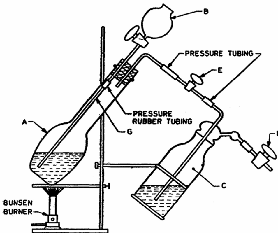
FIG. 2 APPARTUS FOR THE DETERMINATION OF CARBONATES
