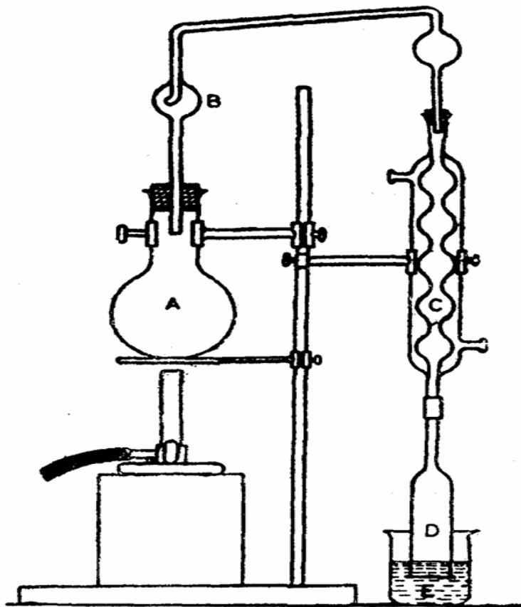
FIG. 1 APPARATUS FOR THE DETERMINATION OF NITRATES
