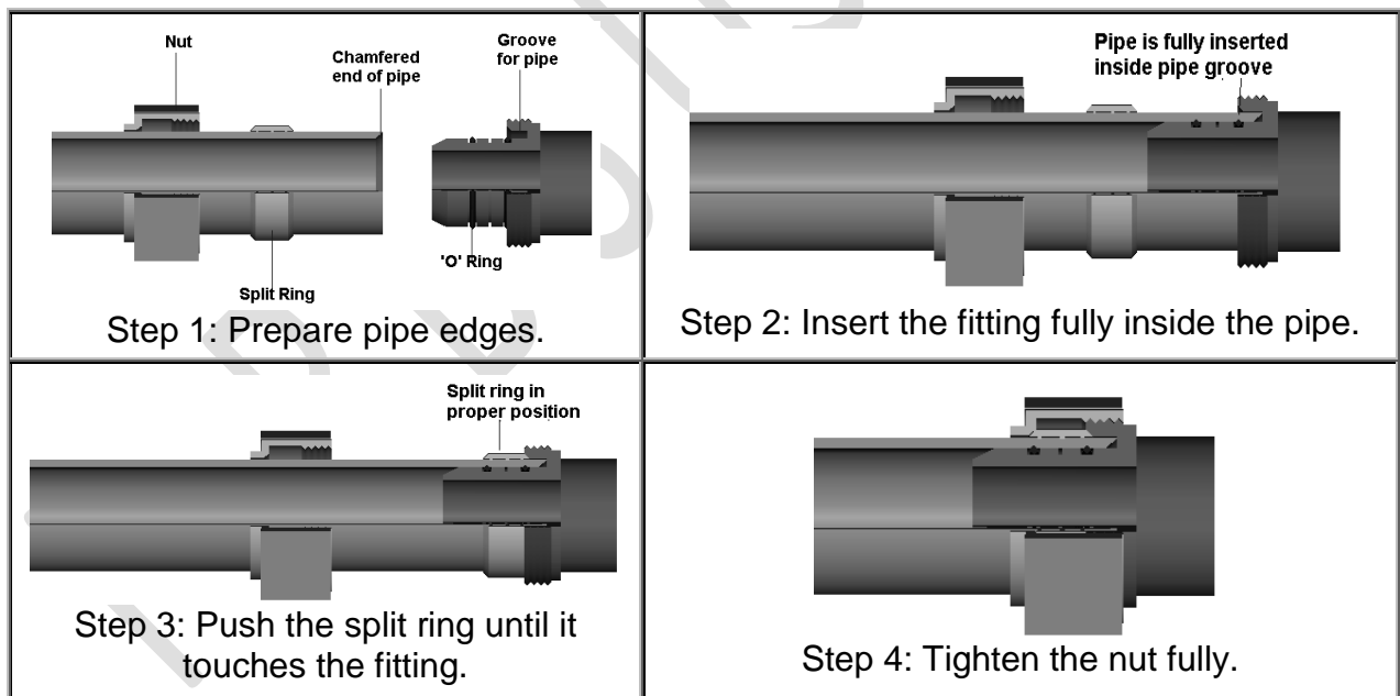
Fig. 13 Jointing using Brass Internal Sealing Fittings
