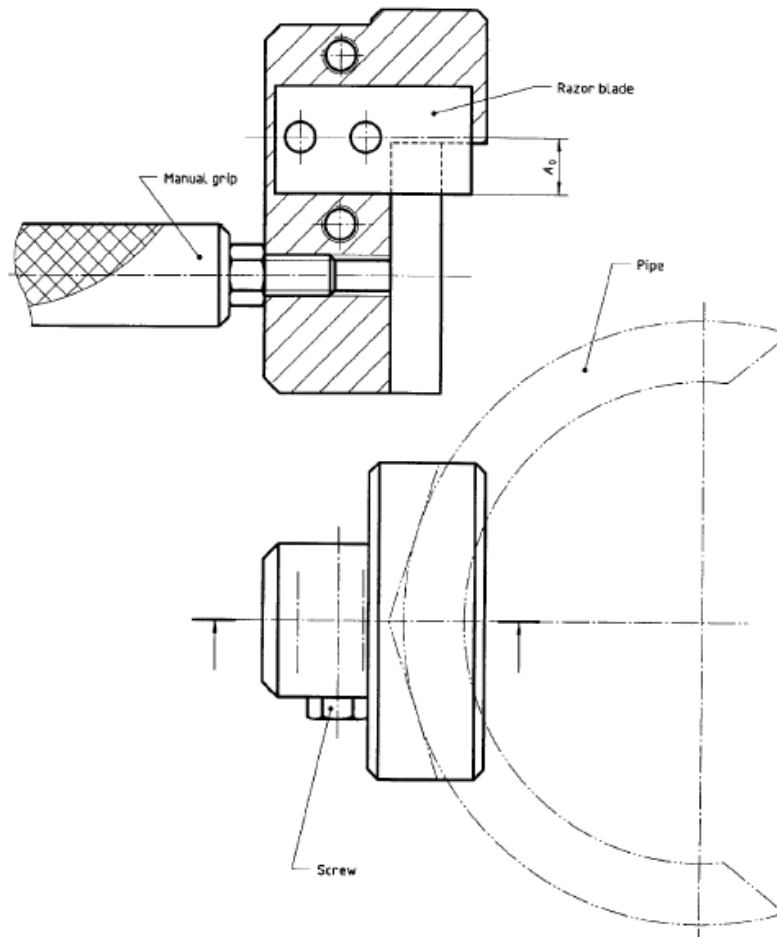
Fig. 4 Notching Device
