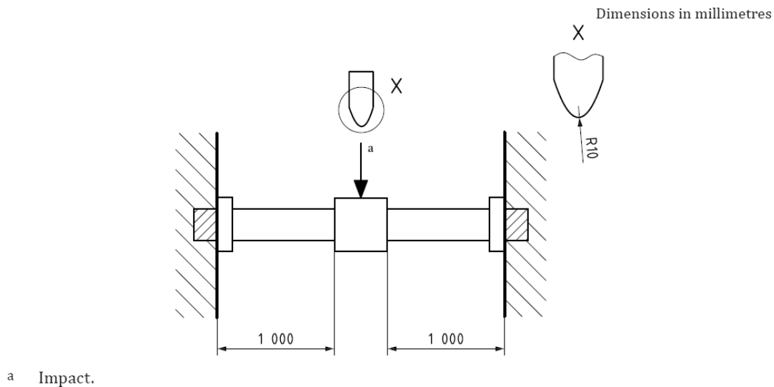
Fig. 9 Impact resistance test assembly
