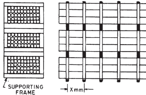
Fig. 12 Stacking Arrangement of Straight length pipes
