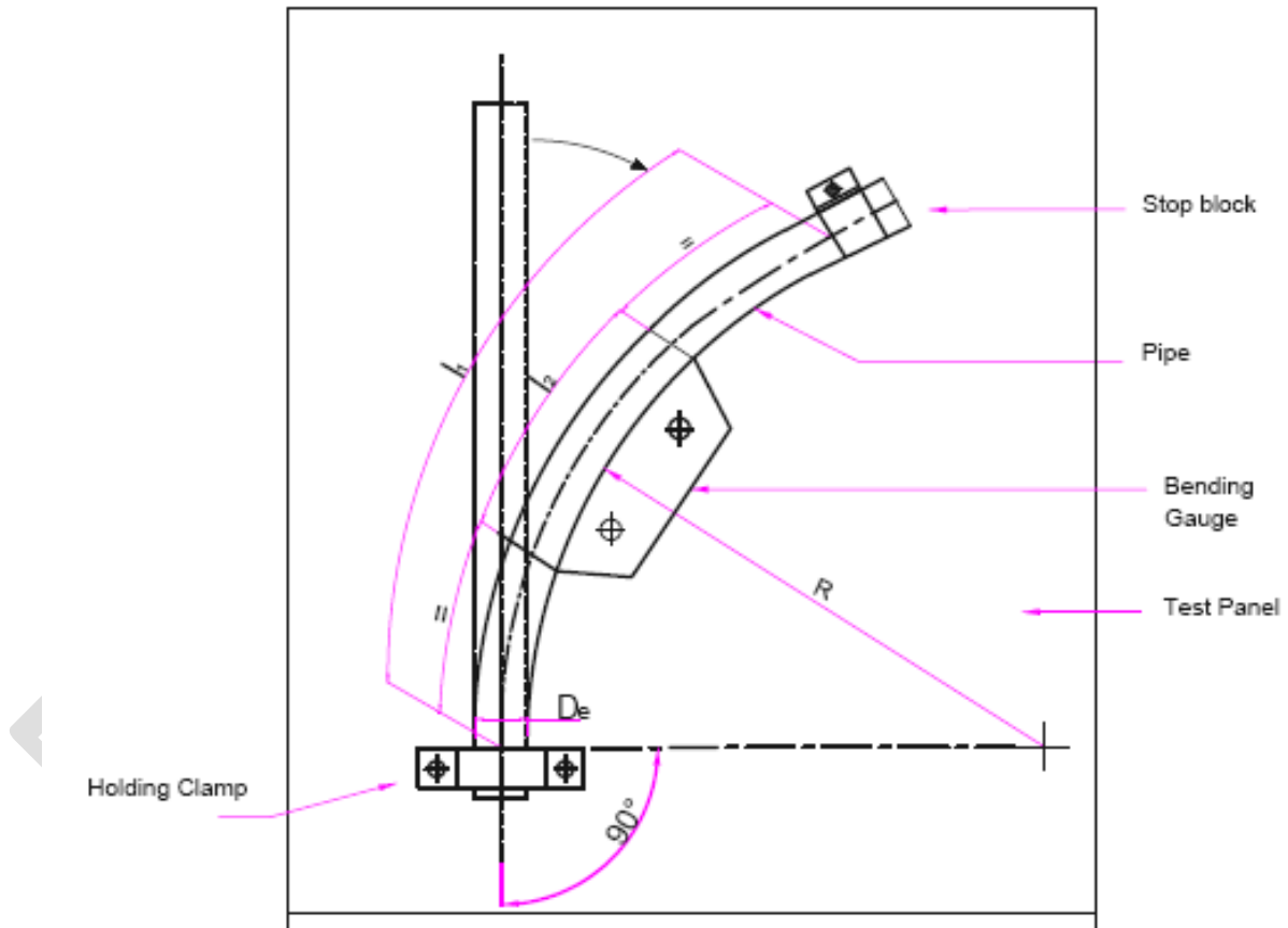
Fig. 6 Diagram of Typical Bending Apparatus
