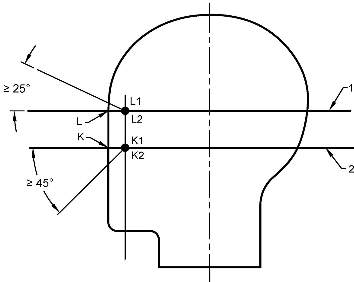
1A SECTION OF HEADFORM IN LONGITUDINAL VERTICAL PLANE
