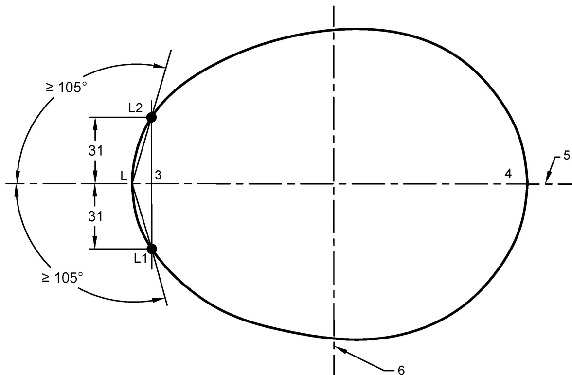
1B SECTION OF HEADFORM IN REFERENCE PLANE
