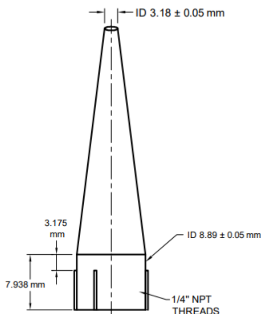
FIG. 1 METAL NOZZLE DIMENSIONS
