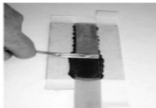
b) WIRE MESS SCREEN BEING IMBEDDED IN WET SEALANT BEAD
