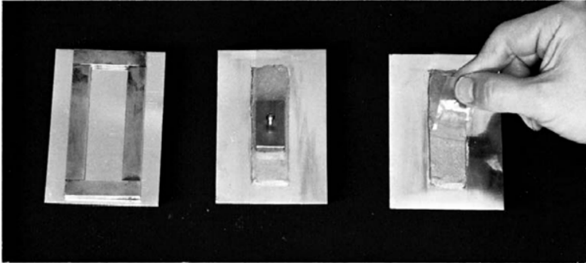
FIG. 5 STAGES IN THE TACK-FREE TIME TEST PROCEDURE
