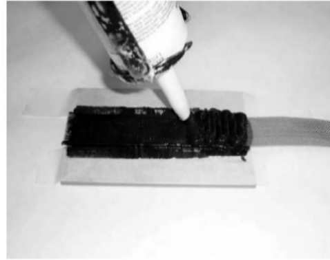
d) TOOLING SECOND BEAD OF SEALANT WITH SPECIAL TOOLING DEVICE–SIDE B
