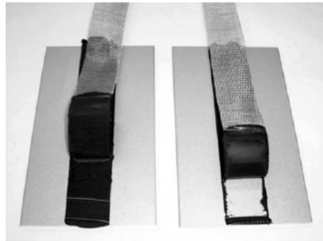
FIG.11 EXAMPLES OF COHESIVE FAILURE AND ADHESIVE FAILURE. LEFT: COHESIVE FAILURE, RIGHT: ADHESIVE FAILURE
