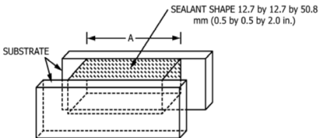
FIG. 18 GLASS SUBSTRATE AND SPACER ASSEMBLED TO FORM A SEALANT CAVITY (TAPE OR CLAMP SUBSTRATES TOGETHER PRIOR TO INJECTING THE SEALANT)
