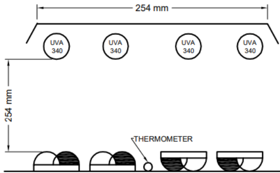
FIG.14 UV EXPOSURE APPARATUS
