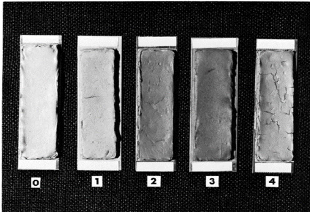
FIG. 3 EXAMPLES OF CRACKING OBTAINABLE IN THIS TEST NUMBER 0 IN THE FIG REPRESENT NO CREAKING.
