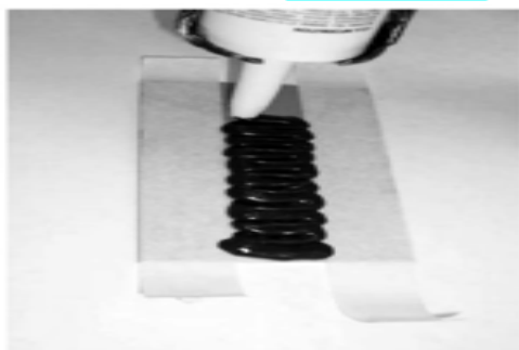
a) FIRST SEALANT BEAD APPLIED TO SUBSTRATE (WITH MASKING TAPE)
