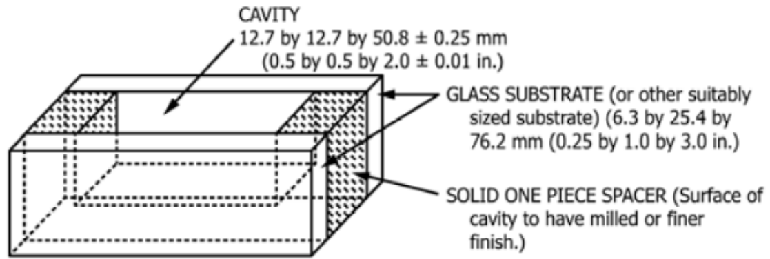
FIG. 16 GLASS SUBSTRATE AND SPACER ASSEMBLED TO FORM A SEALANT CAVITY (TAPE OR CLAMP SUBSTRATES TOGETHER PRIOR TO INJECTING THE SEALANT)
