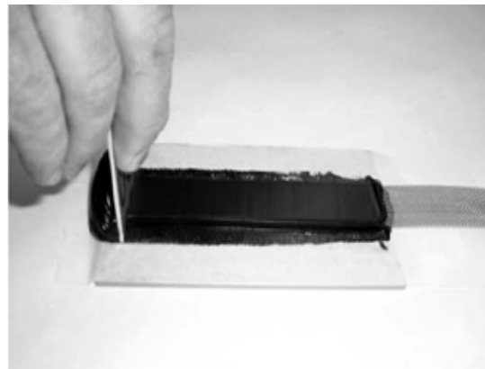
f) TOOLING SECOND BEAD OF SEALANT WITH SPECIAL TOOLING DEVICE–SIDE B
