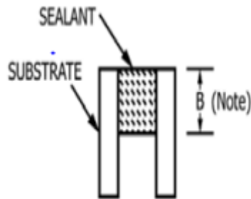
FIG. 17 GLASS SUBSTRATE AND SPACER ASSEMBLED TO FORM A SEALANT CAVITY (TAPE OR CLAMP SUBSTRATES TOGETHER PRIOR TO INJECTING THE SEALANT)
