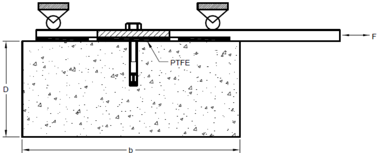
FIG. 5 TYPICAL ALTERNATING SHEAR TEST SETUP
