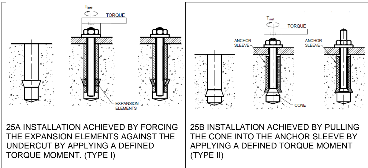
FIG. 25 TORQUE CONTROLLED INSTALLATION – UNDERCUT (MECHANICAL) ANCHORS
