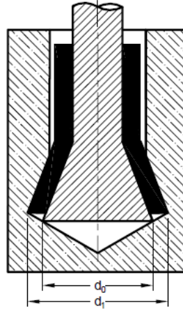
FIG. 12 DIAMETER OF DRILL BIT FOR CYLINDRICAL ( d_0 ) HOLE AND FOR UNDERCUTTING ( d_1 )
