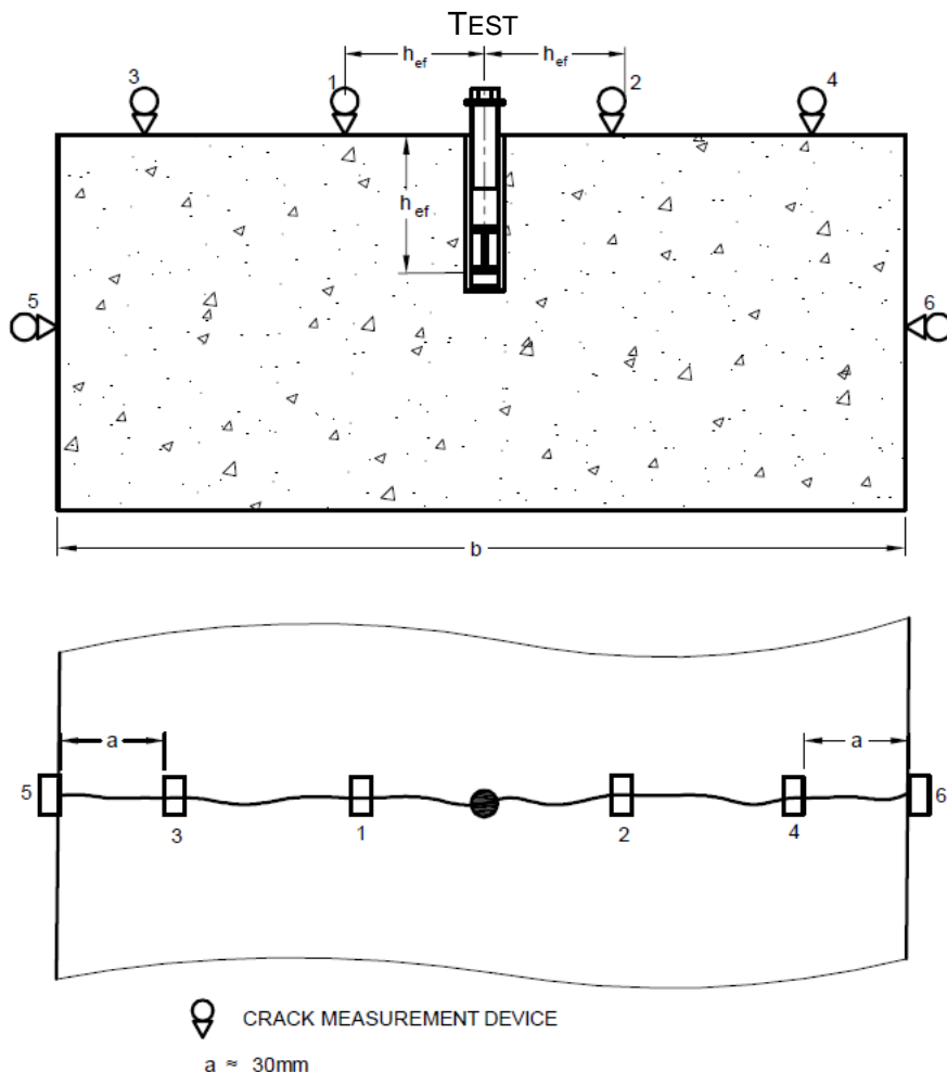
FIG. 8 TYPICAL CRACKED CONCRETE TEST MEMBER AND TEST SET UP FOR CRACK CYCLING
