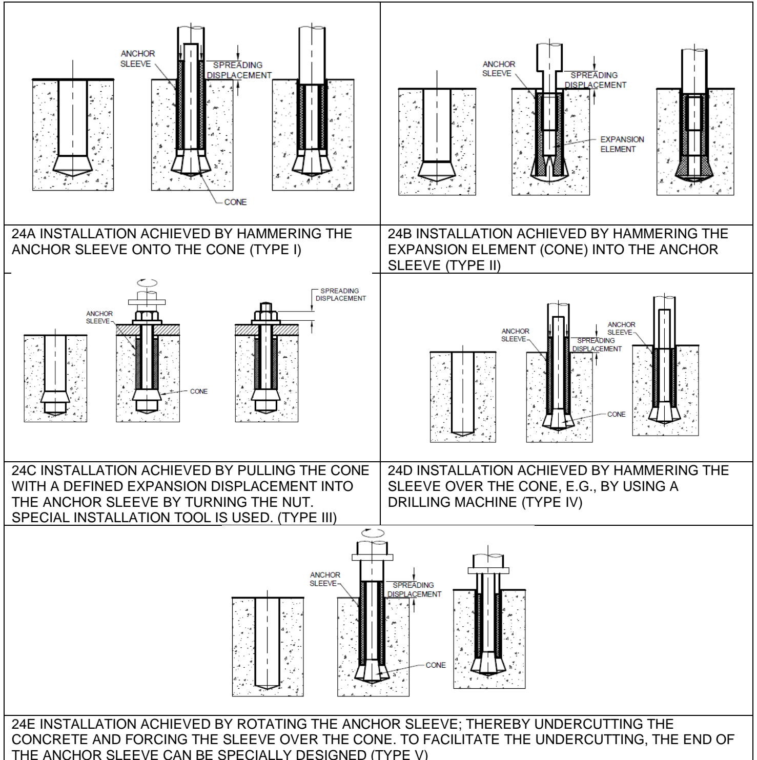
FIG. 24 DISPLACEMENT CONTROLLED INSTALLATION – UNDERCUT (MECHANICAL) ANCHORS
