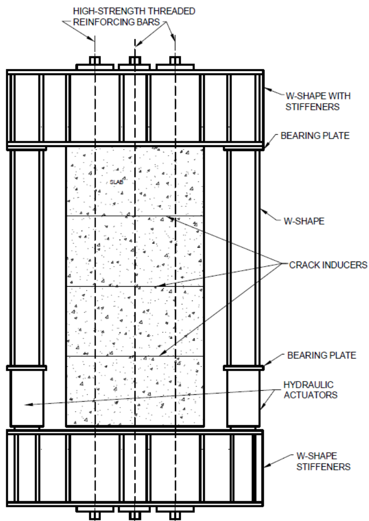
8A Typical cracked concrete test member for crack cycling test
