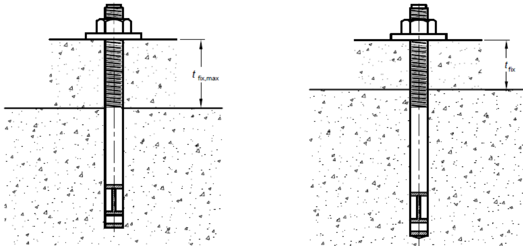
10A Shear plane passing through the smooth shaft of anchor
