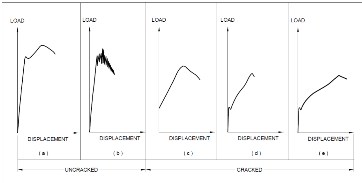
FIG. 27 TYPICAL ACCEPTABLE LOAD DISPLACEMENT BEHAVIOR OF DISPLACEMENT CONTROLLED ANCHORS
