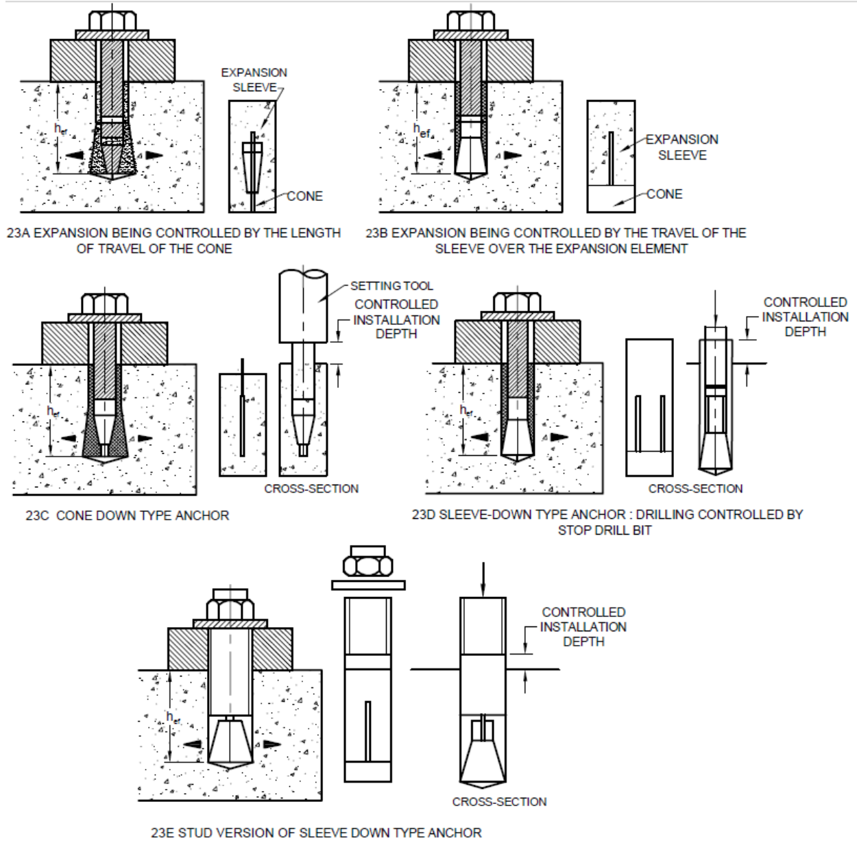
FIG. 23 DISPLACEMENT CONTROLLED EXPANSION ANCHORS
