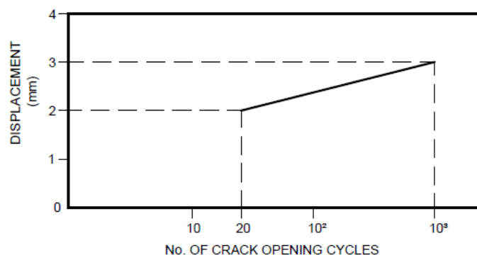
FIG. 20 CRITERIA FOR RESULTS OF TESTS WITH INDUCED CRACKS
