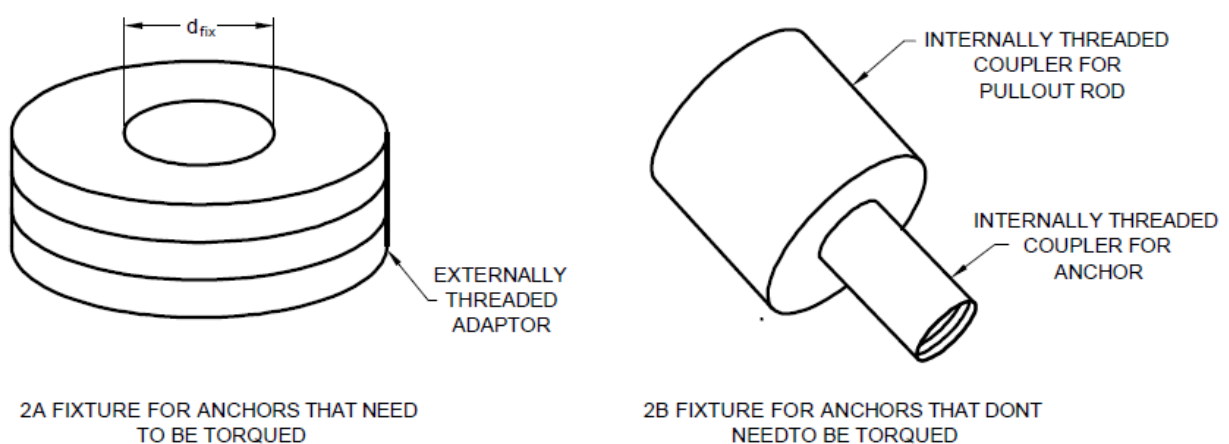
FIG. 2 TYPICAL FIXTURE FOR UNCONFINED TENSION TESTS
