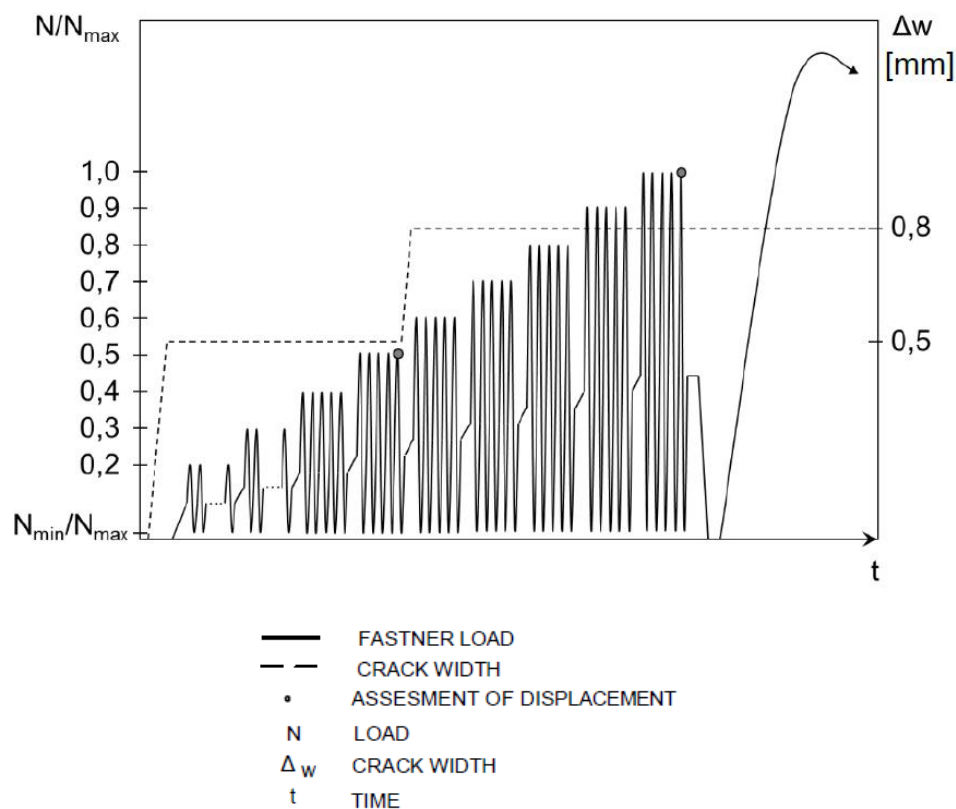
FIG. 15 VARIATION IN TENSION LOAD AMPLITUDE WITH NO. OF CYCLES
