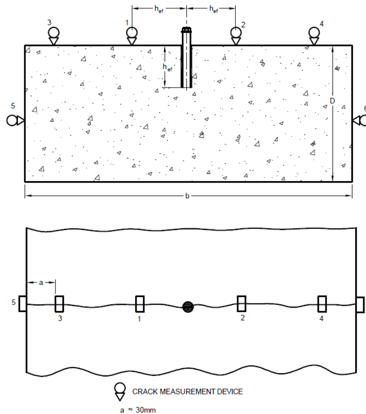
FIG. 11 ILLUSTRATION OF PLACEMENT OF CRACK MEASURING DEVICES TO VERIFY UNIFORM CRACK WIDTH
