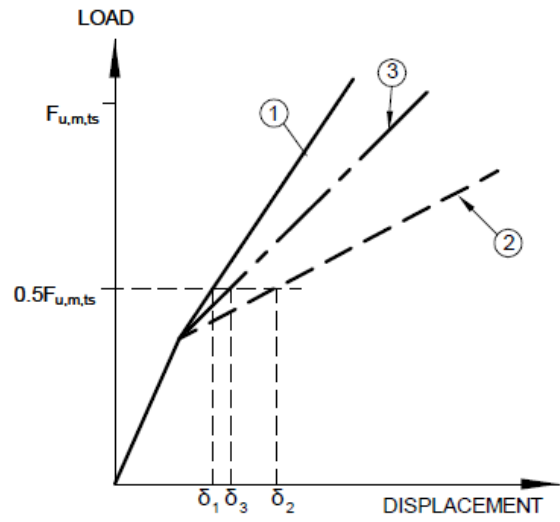
21 B EXAMPLES OF SHIFTING OF CURVES FOR EVALUATION OF SCATTER AT LOAD OF 0.5 F_{u,m,ts}
