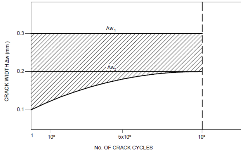
FIG. 14 ALLOWABLE CRACK OPENING VARIATIONS DURING THE CRACK CYCLING TEST
