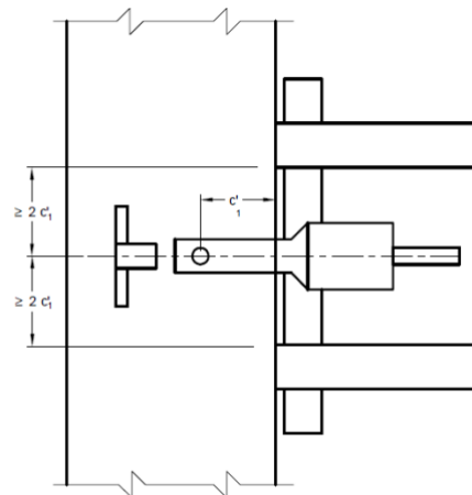
FIG. 4 TYPICAL SHEAR TEST SETUP FIXTURE
