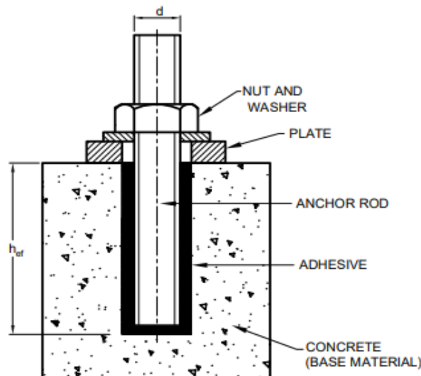
FIG. 7 ADHESIVE ANCHOR
