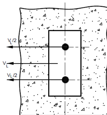
(37A) GROUP OF TWO ANCHORS WHEN LOADED IN SHEAR PARALLEL TO THE EDGE
