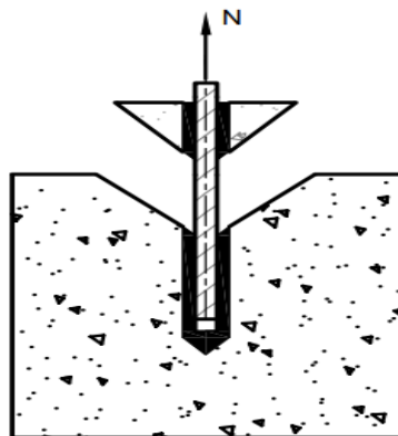
(18 B) BOND FAILURE AT ADHESIVE AND EMBEDDED ELEMENT INTERFACE
