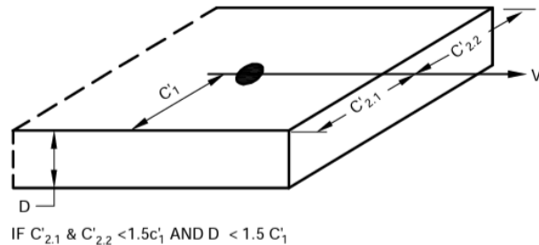
FIG. 51 EXAMPLES OF ANCHORAGE IN A THIN NARROW MEMBER
