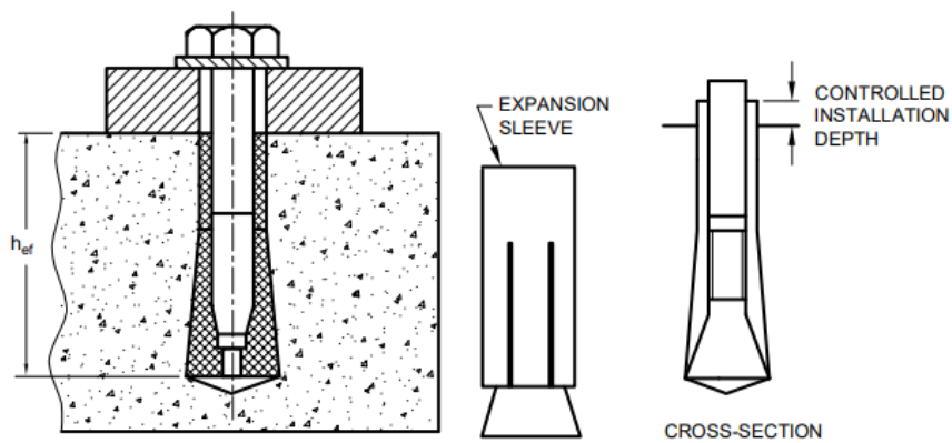
(15C) CONE-DOWN TYPE ANCHOR.
