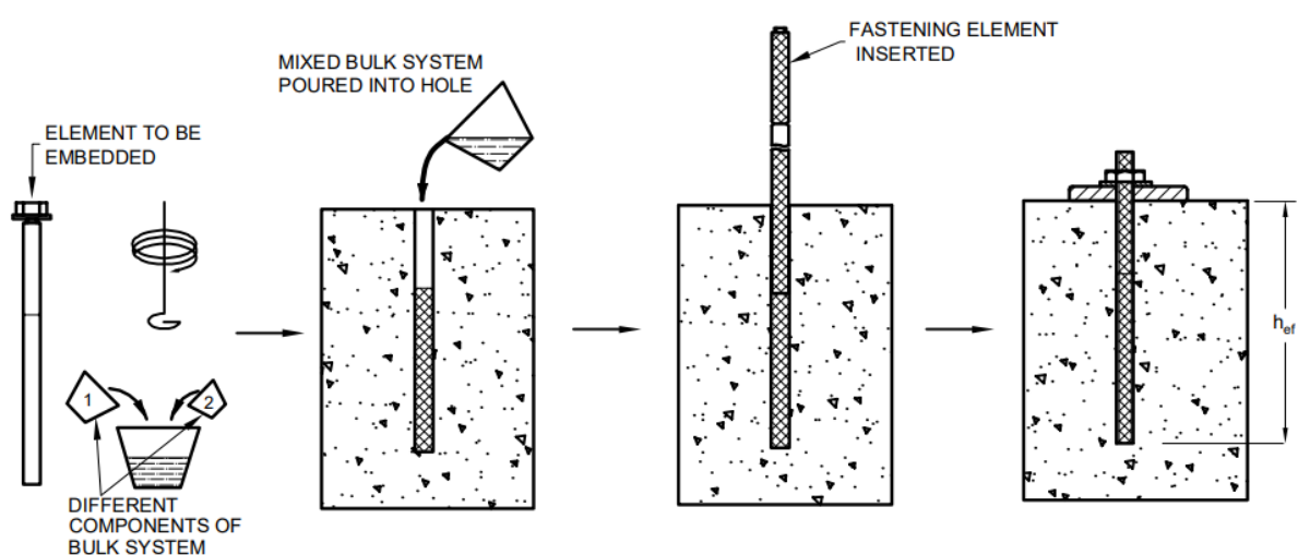
FIG. 10 TYPICAL BULK ADHESIVE SYSTEM
