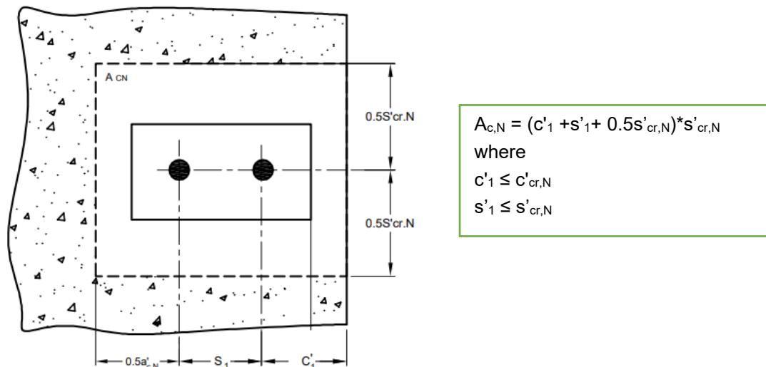
(41B) GROUP OF TWO ANCHORS LOCATED CLOSE TO THE EDGE OF CONCRETE MEMBER
