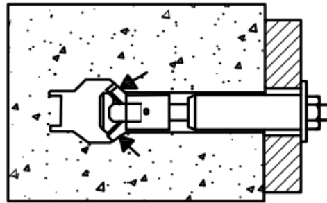
(6A) LOAD TRANSFER DUE TO FRICTION & KEYING BETWEEN METAL PARTS & CONCRETE.
