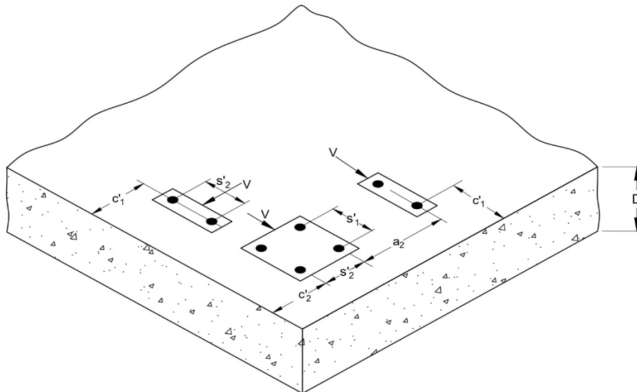
(26B) ANCHOR GROUPS SUBJECTED TO SHEAR LOAD
