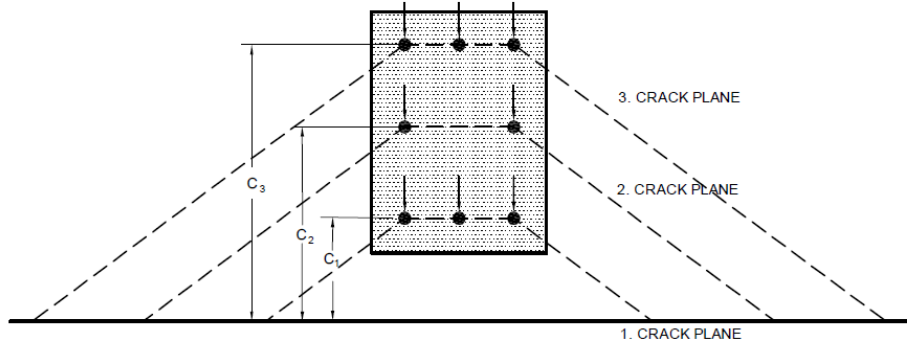
FIG. 48 CRACK PLANES WITH A GROUP OF 8 ANCHORS WITH A SHEAR LOAD PERPENDICULAR TO THE EDGE WITHIN THE RESPECTIVE CRACK PLANE FOR FILLED HOLES
