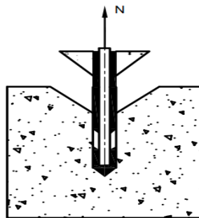
(18 A) BOND FAILURE BASE MATERIAL AND ADHESIVE INTERFACE
