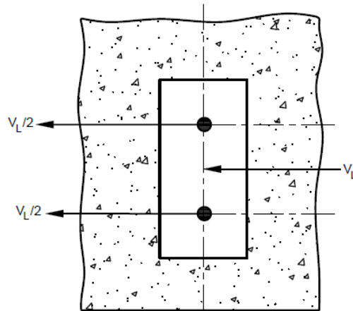
(36A) GROUP OF TWO ANCHORS WHEN LOADED IN SHEAR PARALLEL TO THE EDGE
