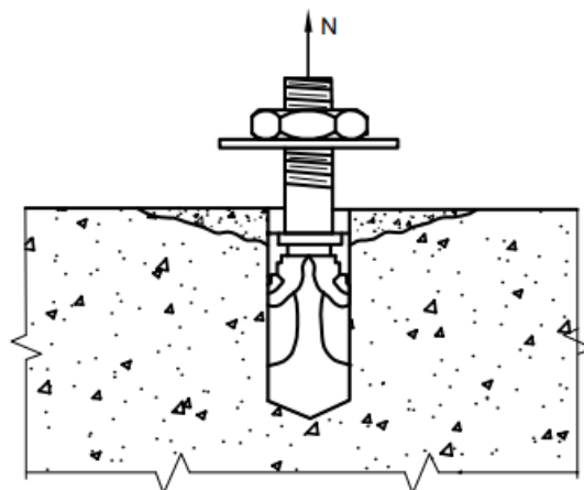
FIG. 22 TYPICAL PULL-OUT FAILURE
