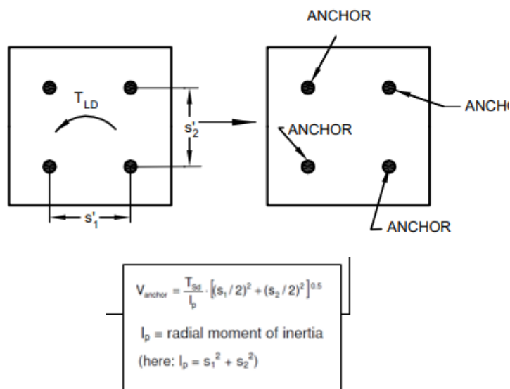
(35D) GROUP OF FOUR ANCHORS SUBJECTED TO TORSION MOMENT
