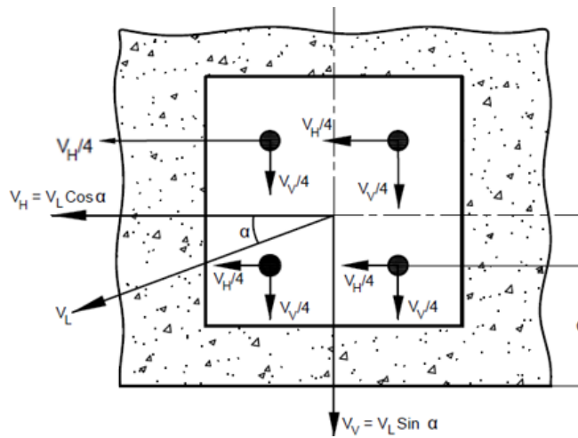
(36B) GROUP OF FOUR ANCHORS WHEN LOADED BY INCLINED SHEAR LOAD
