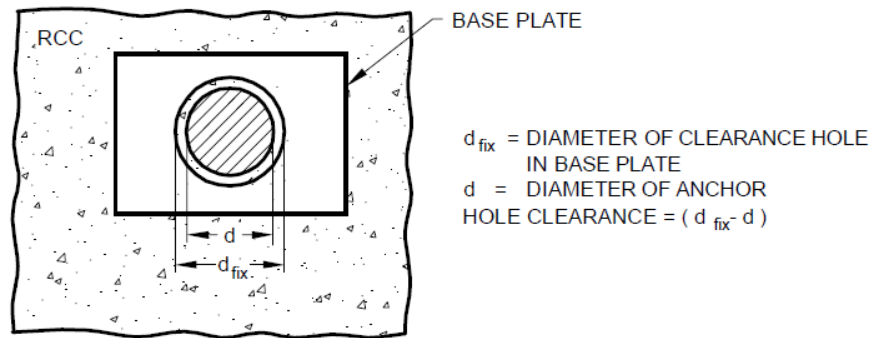
FIG. 5 HOLE CLEARANCE
