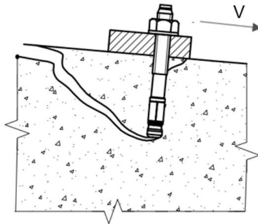
FIG. 21 TYPICAL CONCRETE PRY-OUT FAILURE
