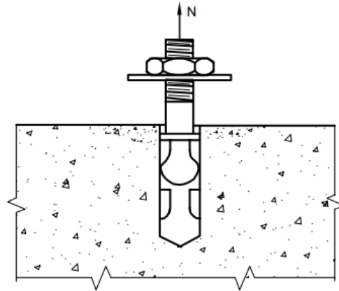
FIG. 23 TYPICAL PULL-THROUGH FAILURE
