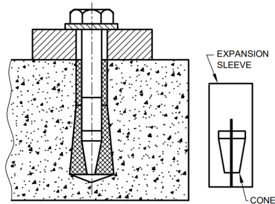
(15A) EXPANSION BEING CONTROLLED BY LENGTH OF TRAVEL OF THE CONE.
