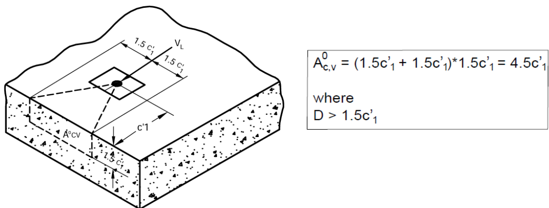
FIG. 46 IDEALIZED PROJECTED CONCRETE CONE AREA, A_{c,v}^0 OF AN INDIVIDUAL ANCHOR
