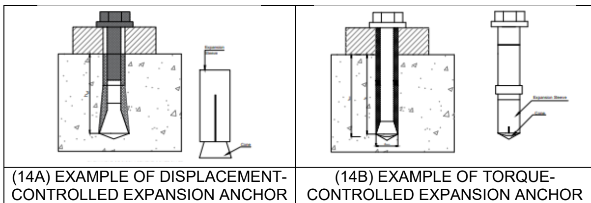
FIG. 14 DIFFERENT TYPES OF EXPANSION ANCHORS.
