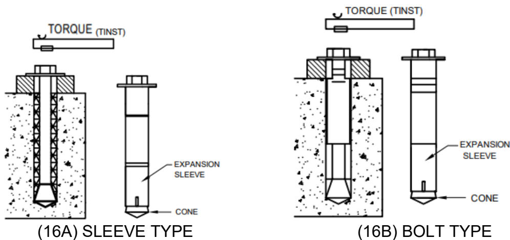
FIG. 16 TYPICAL TORQUE-CONTROLLED EXPANSION ANCHOR
