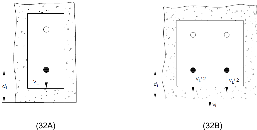
FIG. 32 EXAMPLE OF DISTRIBUTION OF SHEAR LOAD - ANCHOR LOCATED NEAR THE EDGE (WHEN GAP BETWEEN THE ANCHOR AND THE BASE PLATE IS NOT FILLED UP)
