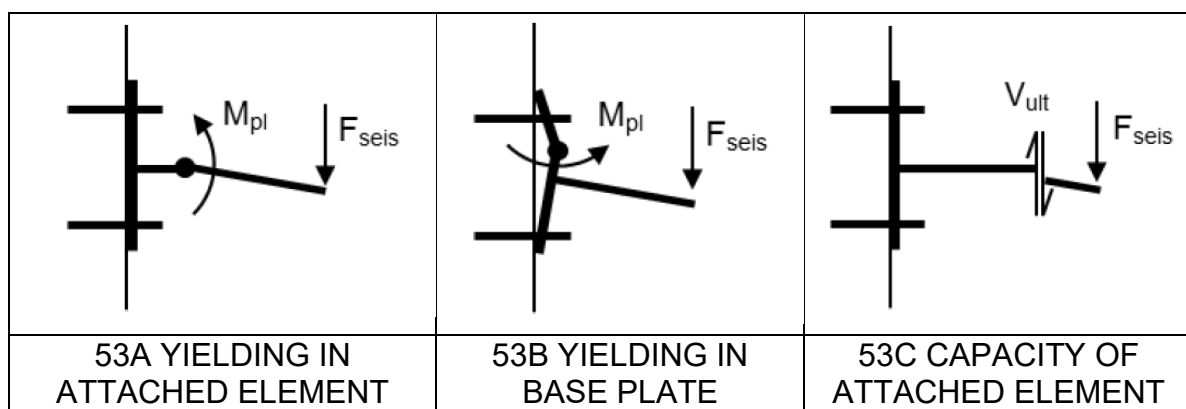
FIG. 53 SEISMIC DESIGN BY PROTECTION OF ANCHOR (see 10.2.1 )
