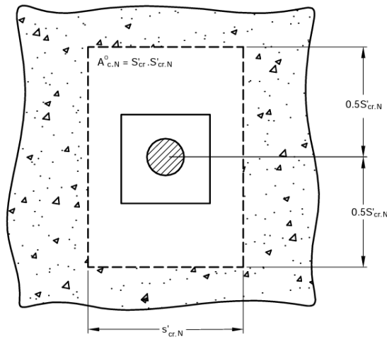
FIG. 40 IDEALIZED PROJECTED CONE AREA OF AN INDIVIDUAL ANCHOR
