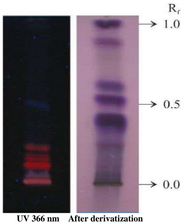
Fig. 2: TLC fingerprints of Shakh-i-Thuhar ( Euphorbia neriiifolia L.) Stem
