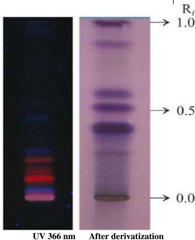
Fig. 3: TLC fingerprints of Shakh-i-Thuhar ( Euphorbia nerifolia L.) Stem
