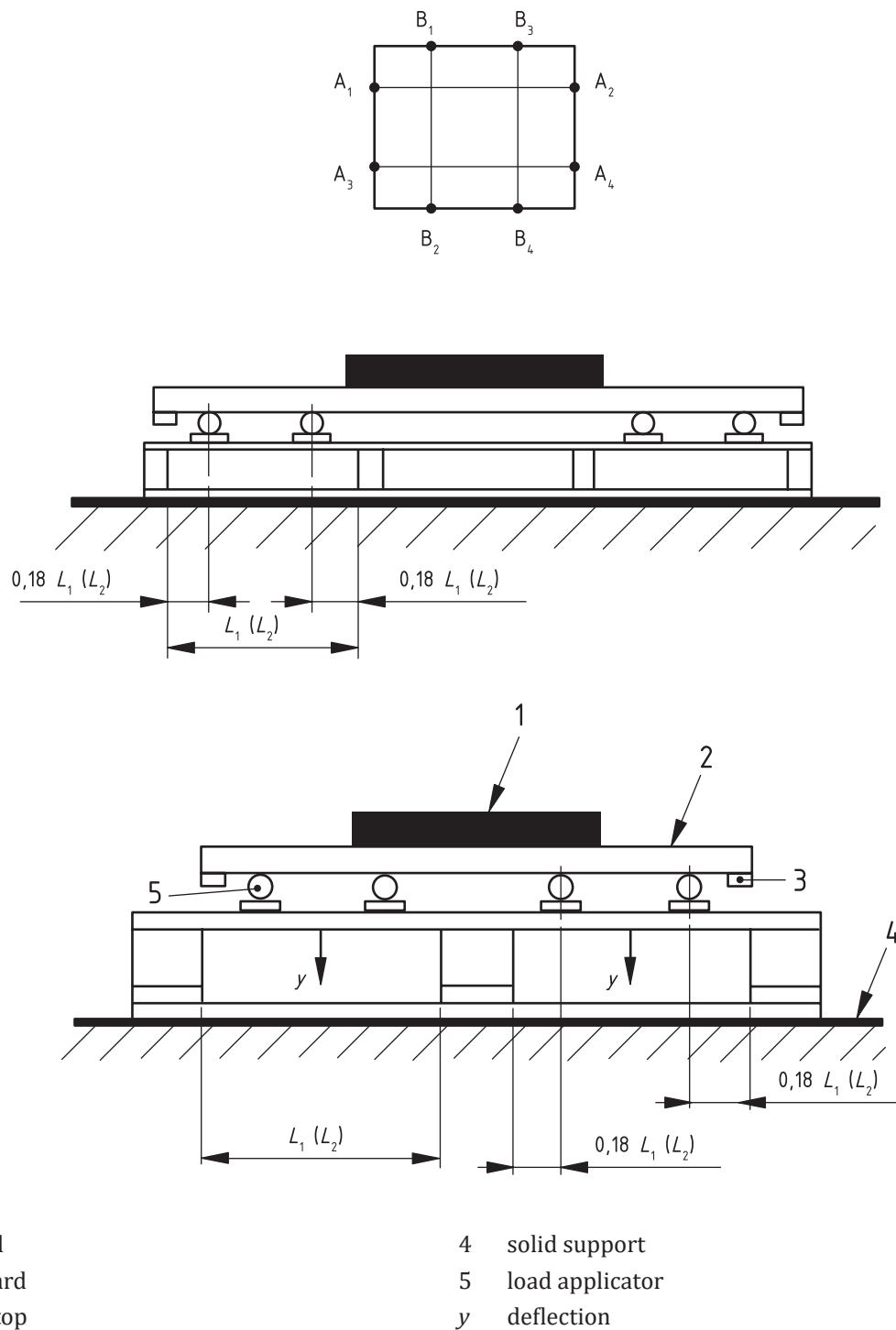
Figure 4 — Deck strength and stiffness test
