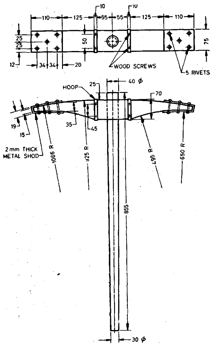
FIG. 3 WOODEN BEATER, TAPER FACED, METAL SHOD
