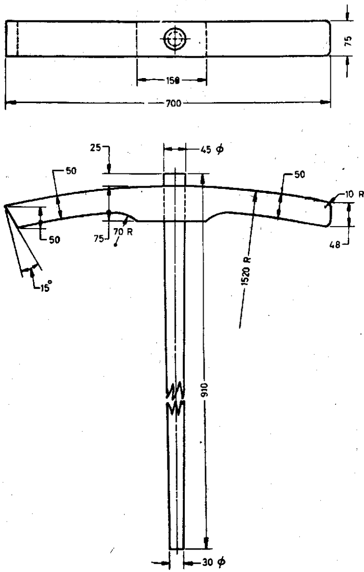
FIG. 1 WOODEN BEATER, FLAT FACED
