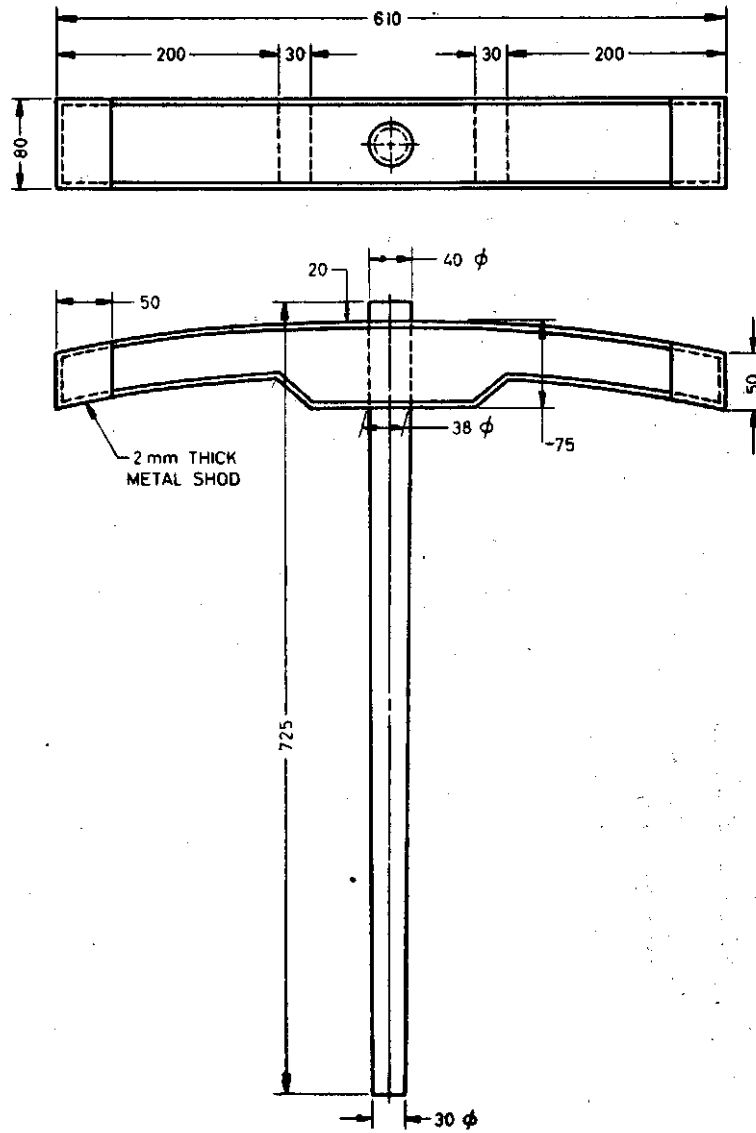
FIG. 2 WOODEN BEATER, FLAT FACED, METAL SHOD
