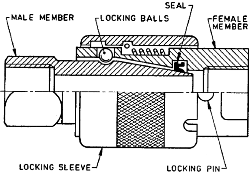
FIG. 2 FEMALE MEMBER
