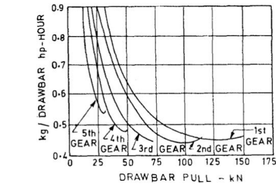
B-SPECIFIC FUEL CONSUMPTION/PULL
