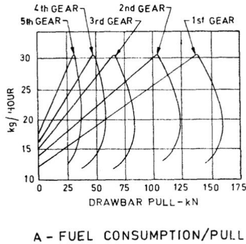
FIG. 3 DRAWBAR TEST CURVES FORWARD SPEED/PULL GRASSLAND ON HEAVY CLAY
