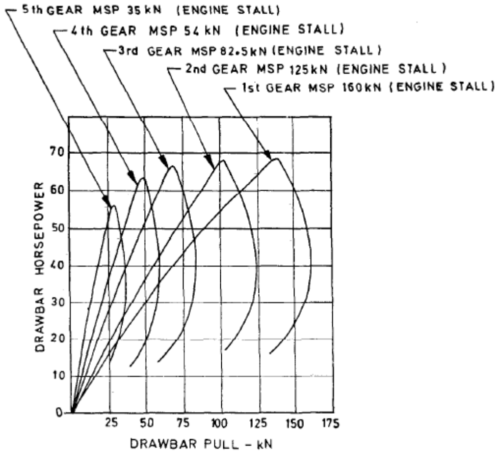
A - DRAWBAR HORSEPOWER/PULL
