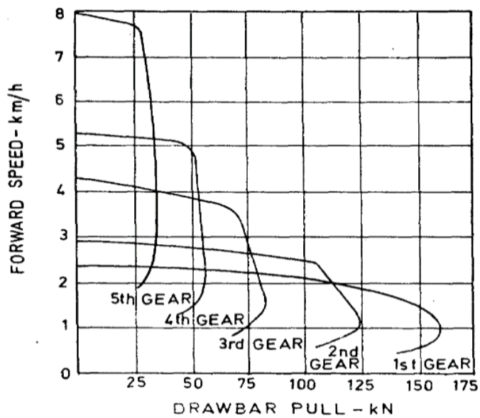
FIG. 2 Drawbar Test Curves, Grassland on Heavy Clay
