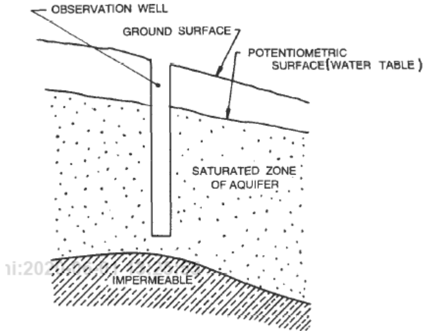
FIG. 1 OBSERVATION WELL IN AN UNCONFINED AQUIFER
