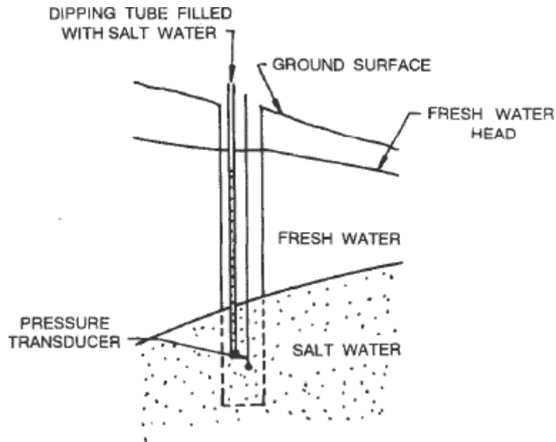
FIG. 3 OBSERVATION WELL PENETRATING SALT WATER
