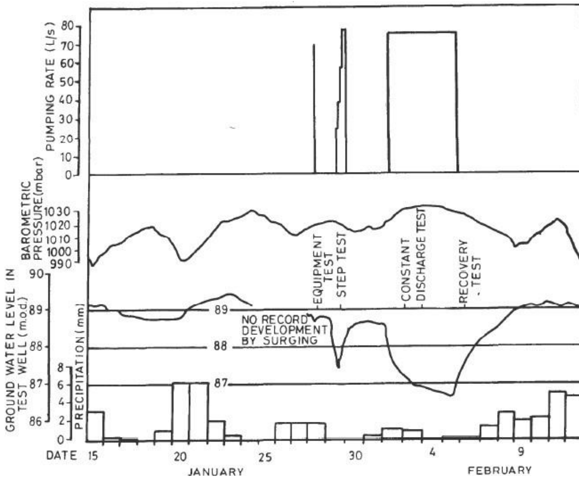
FIG. 2 CONTINUOUS PLOT OF PUMPING TEST DATA
