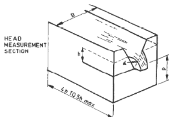
Fig. 1 V- Notch Thin Plate Weir
