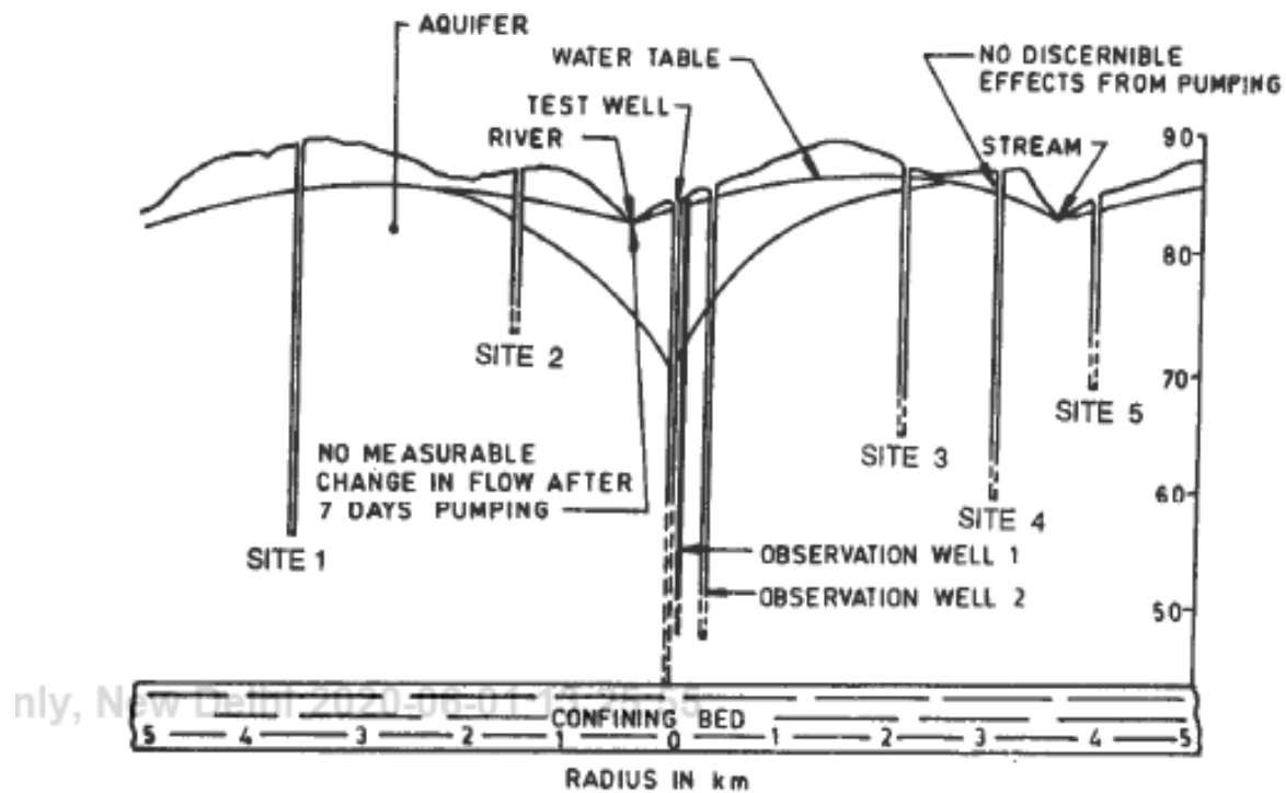
Fig. 1 TYPICAL VERTICAL SECTION THROUGH TEST WELL AND ENVIRONS
