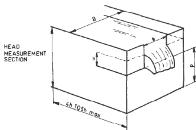
Fig. 2 Rectangular Notch Thin Plat Weir
