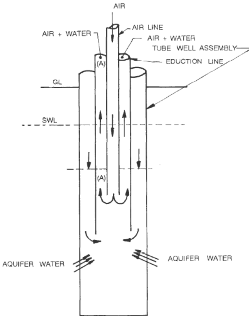
Fig. 3 DEVELOPMENT OF COMPRESSED AIR
