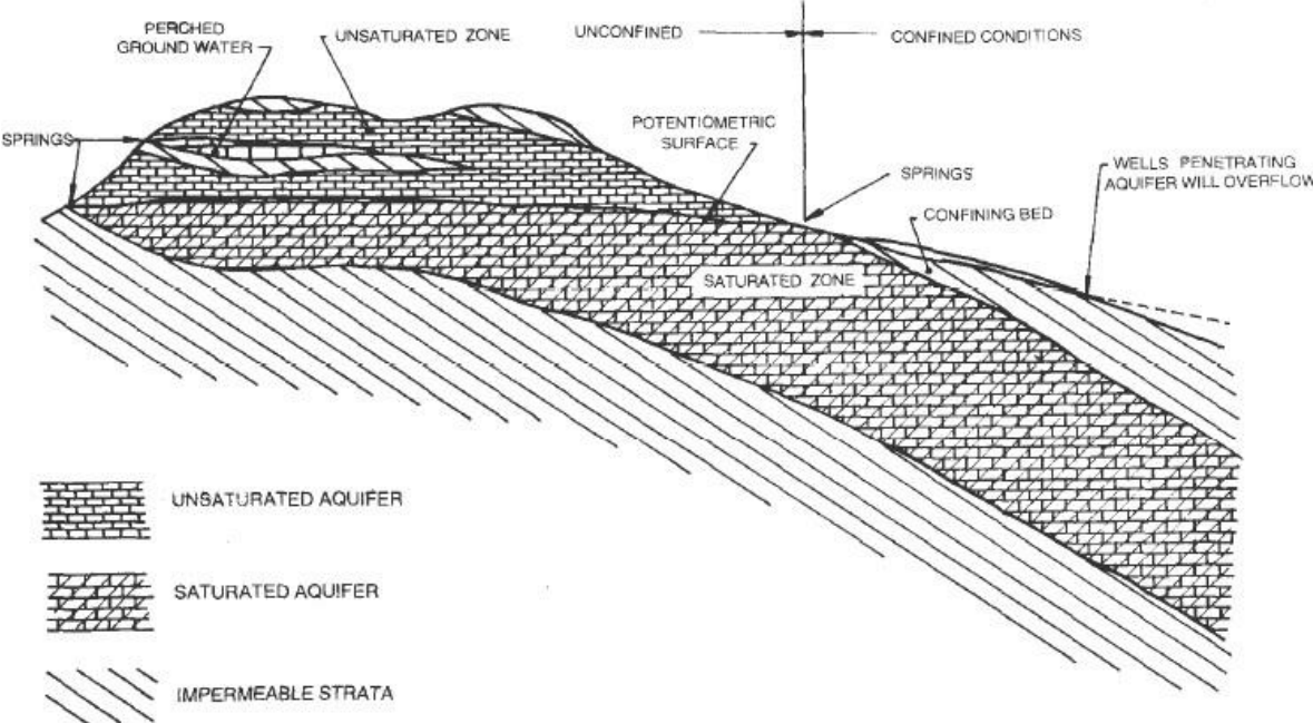
FIG. 1 GROUNDWATER CONDITIONS AND AQUIFER STATES
