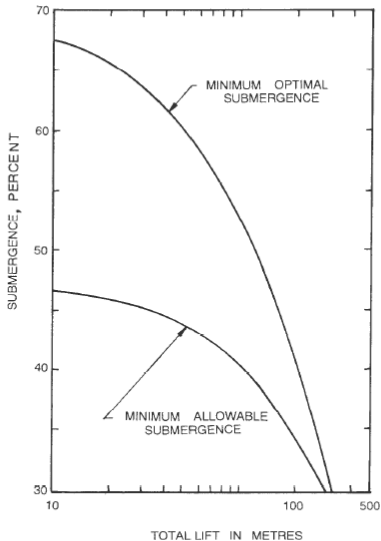
FIG. 2 DEGREE OF SUBMERGENCE REQUIRED FOR AIRLIFT PUMPS
