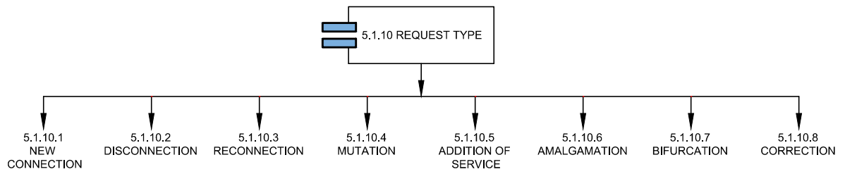
FIG. 5 TAXONOMY OF REQUEST TYPE
