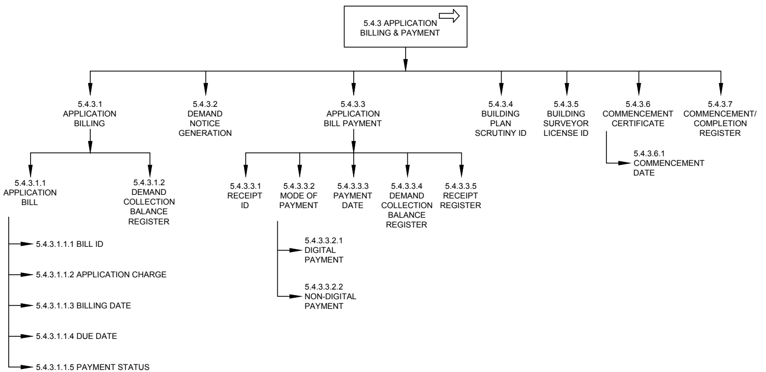
FIG. 22 TAXONOMY FOR APPLICATION BILLING AND PAYMENT PROCESS
