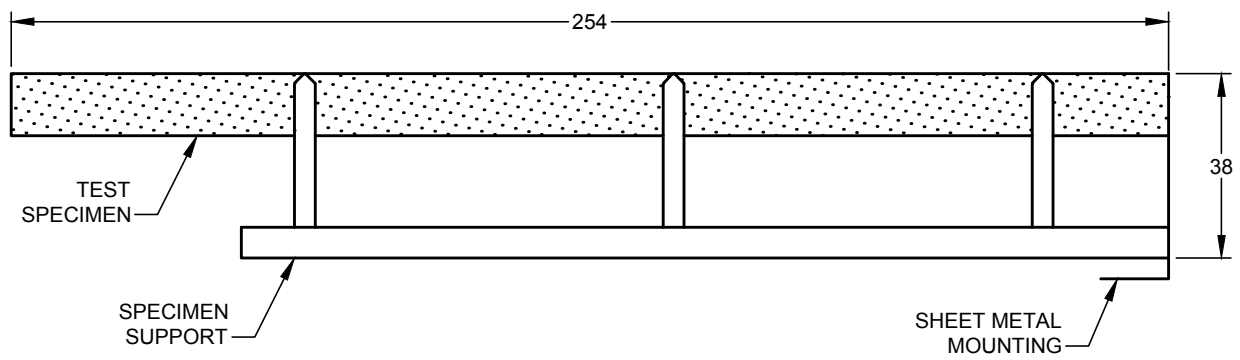
FIG. 3 TEST SPECIMEN INPOLED ON SPECIMEN SUPPORT (SIDE VIEW)
